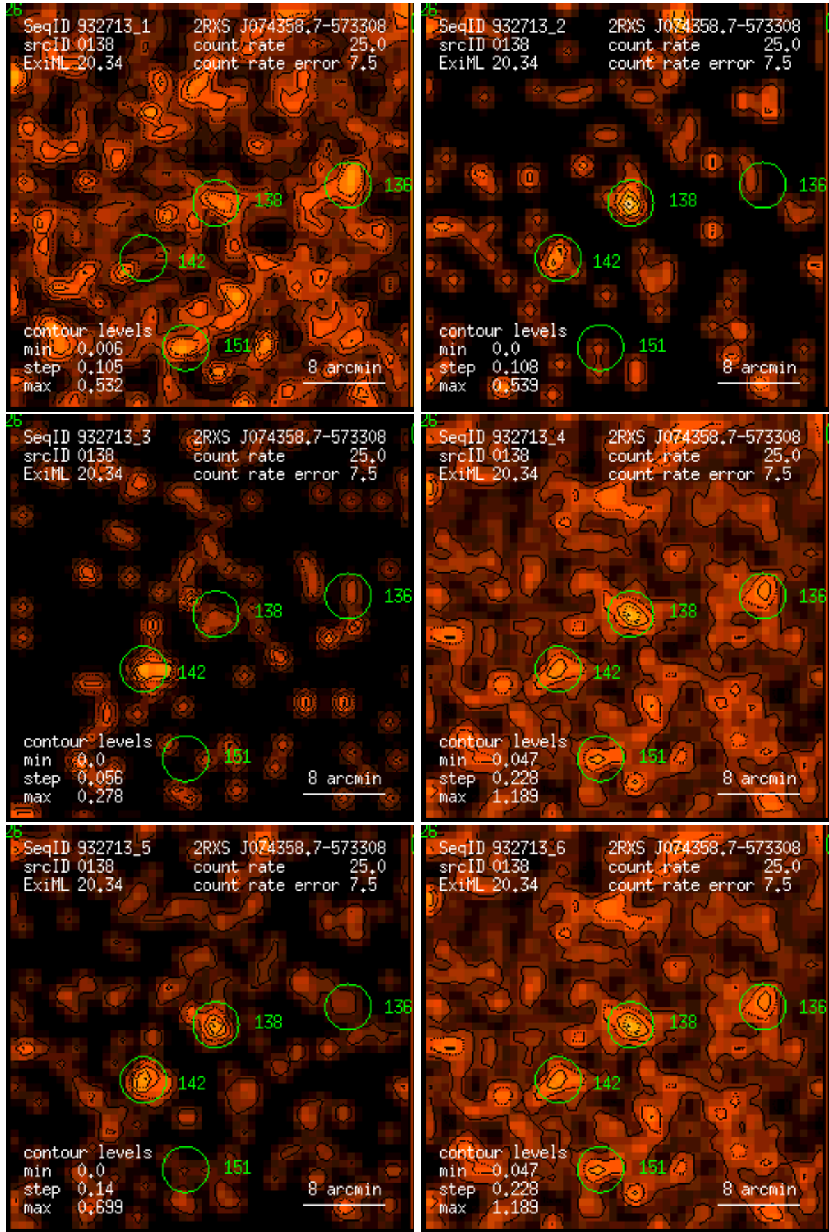
Figure 138: RASS 932713: detection 0138: band rate images, Gaussian filter: (1) PSPC channels 11 – 41, (2) 52 – 90, (3) 91 – 201, (4) 11 – 235, (5) 52 – 201, (6) 11 – 201. Broad band rates in counts/ks. Band rate contour levels in counts/ks/arcmin 2 .
