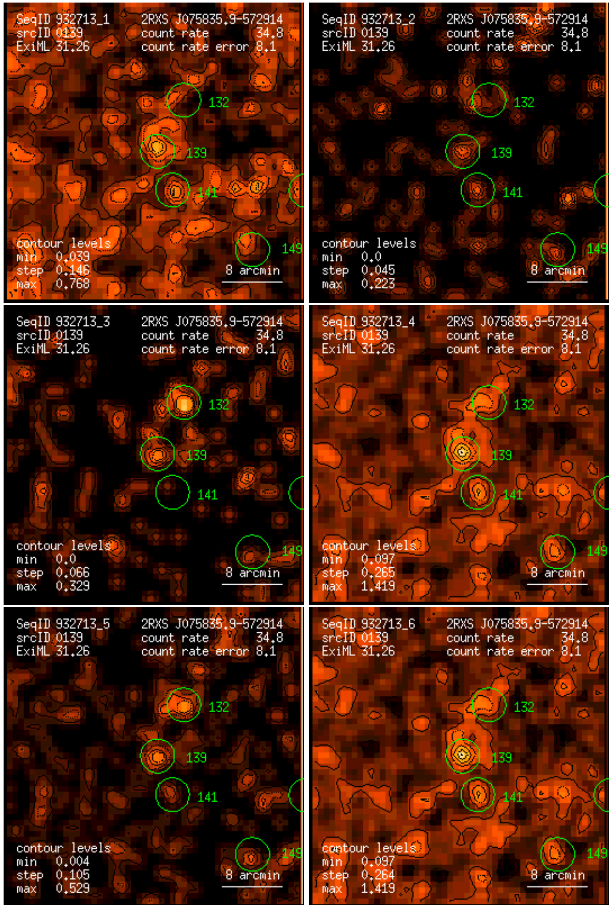
Figure 139: RASS 932713: detection 0139: band rate images, Gaussian filter: (1) PSPC channels 11 – 41, (2) 52 – 90, (3) 91 – 201, (4) 11 – 235, (5) 52 – 201, (6) 11 – 201. Broad band rates in counts/ks. Band rate contour levels in counts/ks/arcmin 2 .
