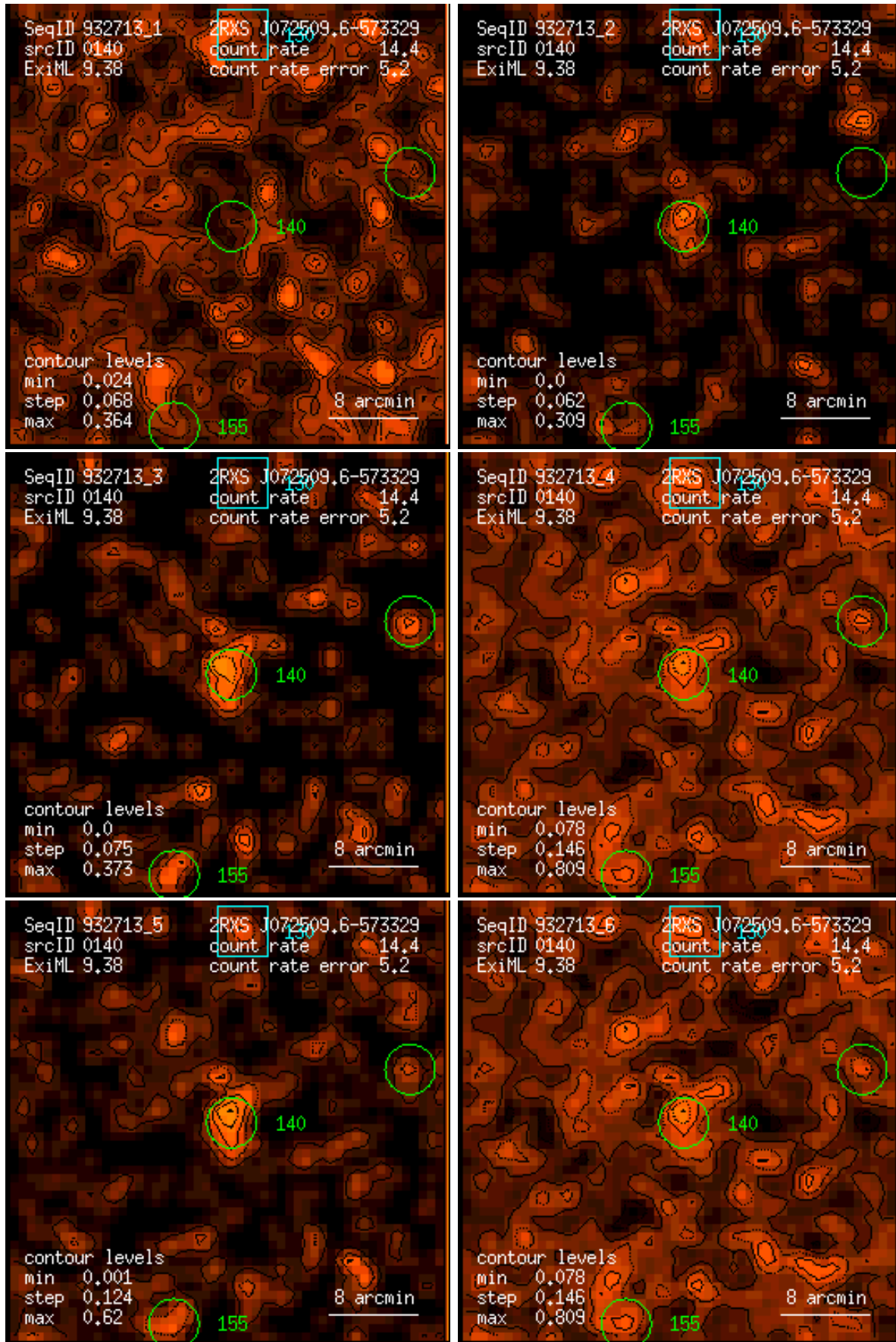
Figure 140: RASS 932713: detection 0140: band rate images, Gaussian filter: (1) PSPC channels 11 – 41, (2) 52 – 90, (3) 91 – 201, (4) 11 – 235, (5) 52 – 201, (6) 11 – 201. Broad band rates in counts/ks. Band rate contour levels in counts/ks/arcmin 2 .
