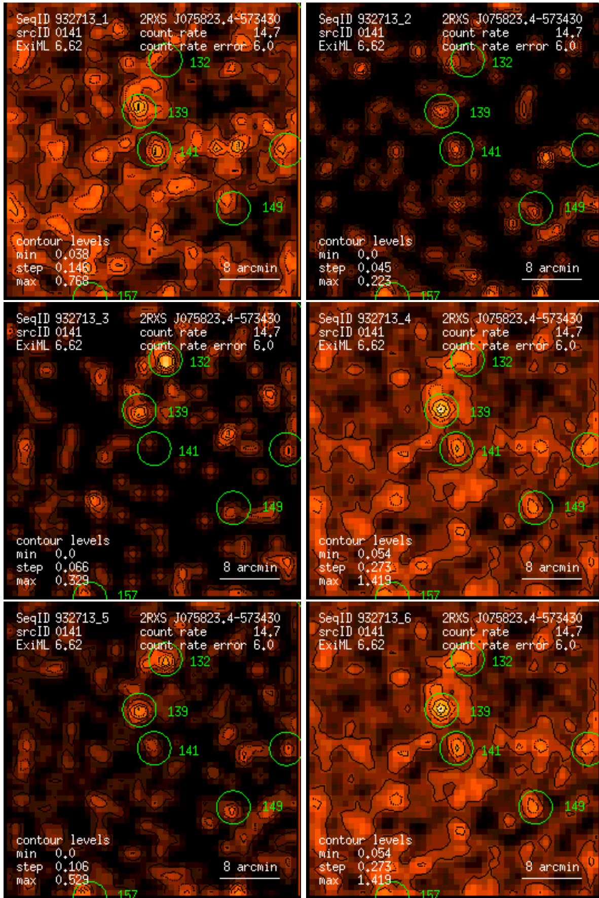
Figure 141: RASS 932713: detection 0141: band rate images, Gaussian filter: (1) PSPC channels 11 – 41, (2) 52 – 90, (3) 91 – 201, (4) 11 – 235, (5) 52 – 201, (6) 11 – 201. Broad band rates in counts/ks. Band rate contour levels in counts/ks/arcmin 2 .
