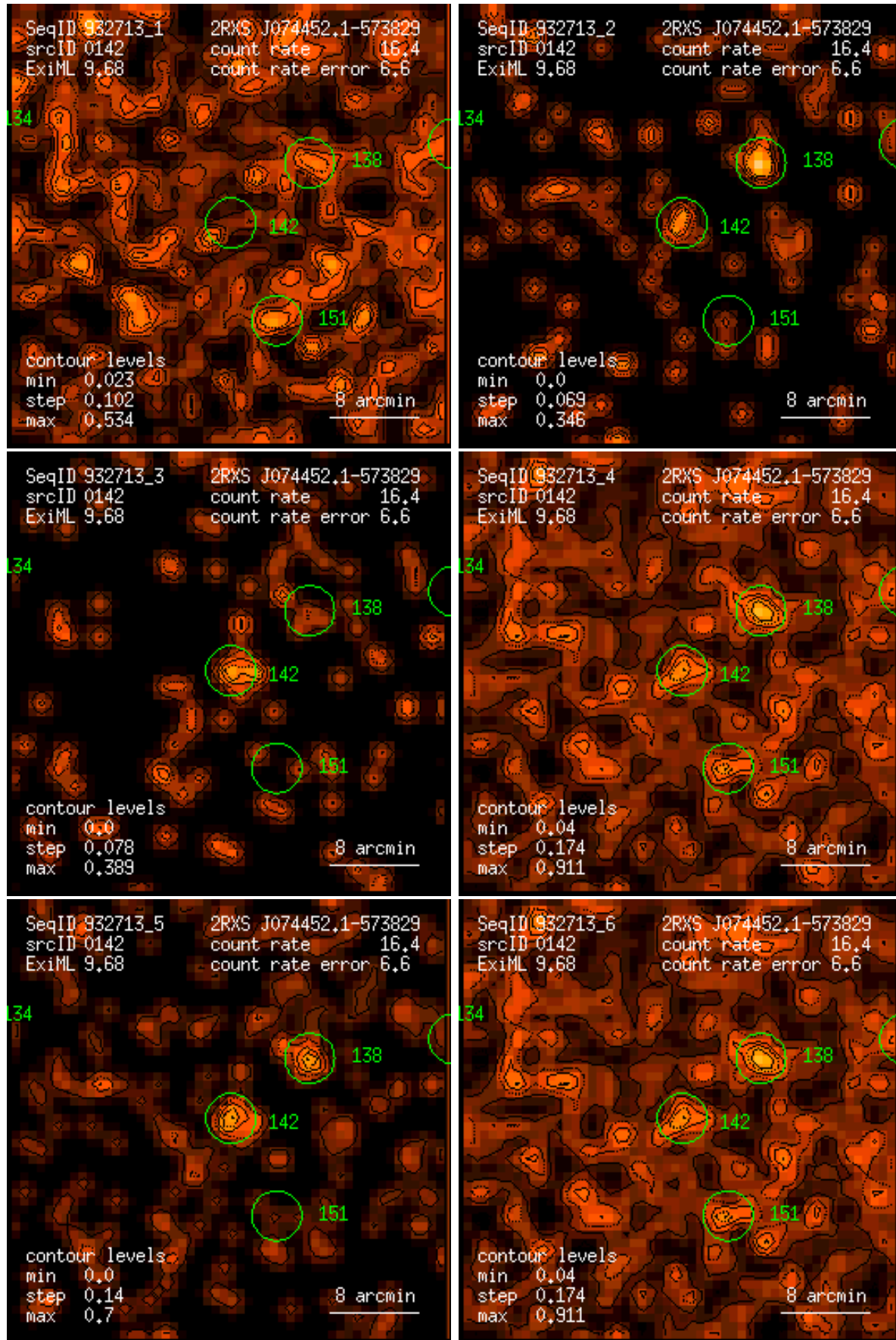
Figure 142: RASS 932713: detection 0142: band rate images, Gaussian filter: (1) PSPC channels 11 – 41, (2) 52 – 90, (3) 91 – 201, (4) 11 – 235, (5) 52 – 201, (6) 11 – 201. Broad band rates in counts/ks. Band rate contour levels in counts/ks/arcmin 2 .
