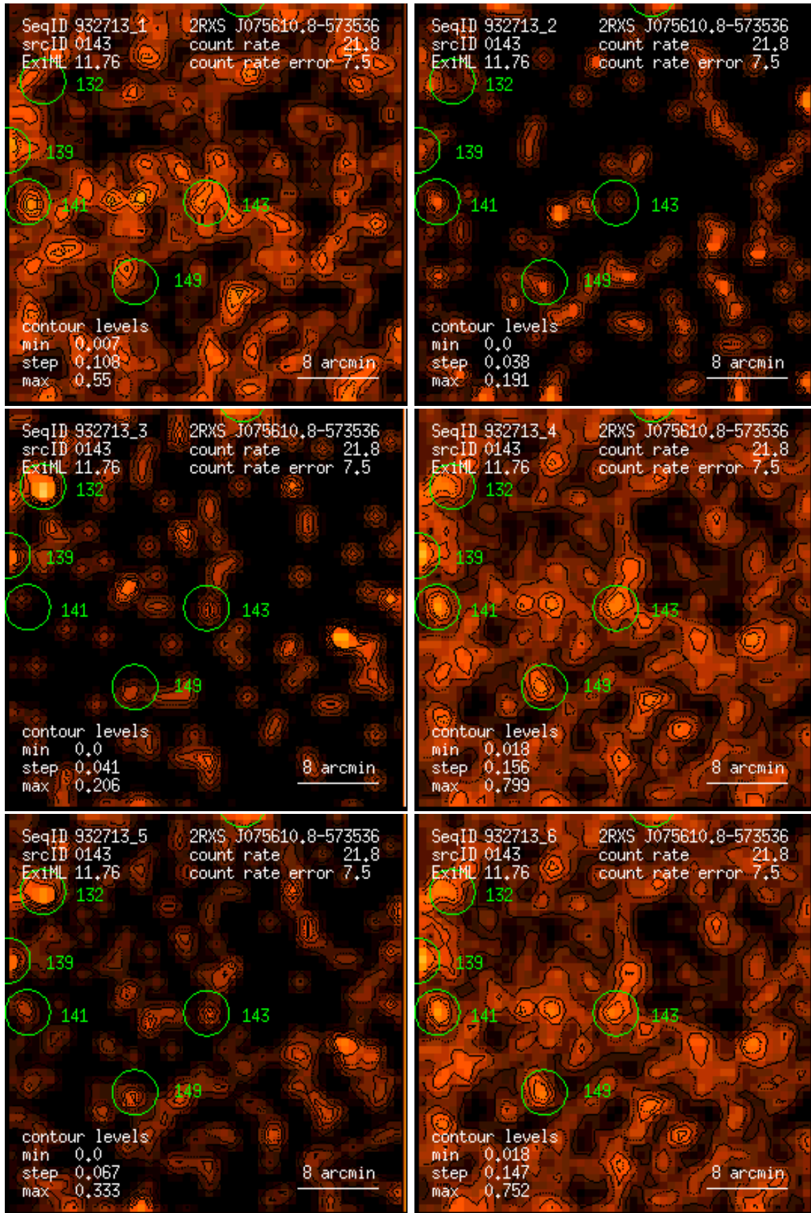
Figure 143: RASS 932713: detection 0143: band rate images, Gaussian filter: (1) PSPC channels 11 – 41, (2) 52 – 90, (3) 91 – 201, (4) 11 – 235, (5) 52 – 201, (6) 11 – 201. Broad band rates in counts/ks. Band rate contour levels in counts/ks/arcmin 2 .
