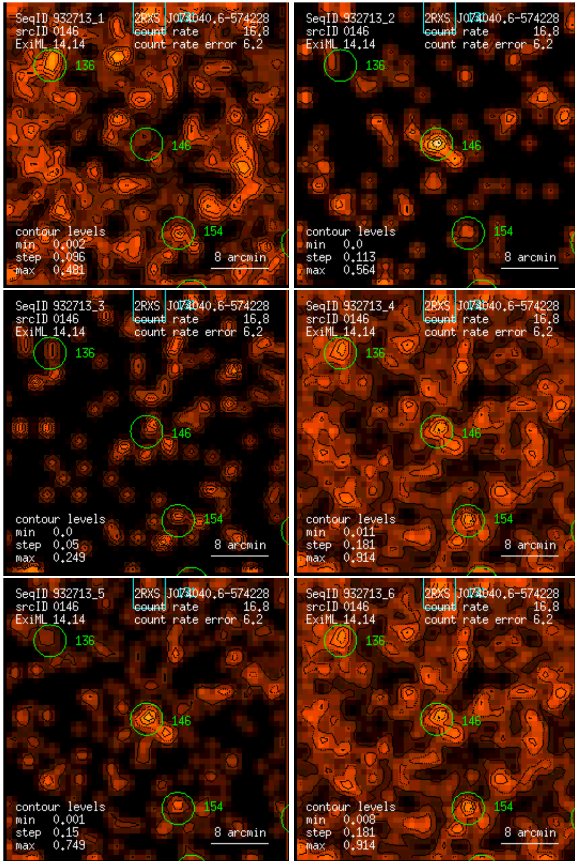
Figure 146: RASS 932713: detection 0146: band rate images, Gaussian filter: (1) PSPC channels 11 – 41, (2) 52 – 90, (3) 91 – 201, (4) 11 – 235, (5) 52 – 201, (6) 11 – 201. Broad band rates in counts/ks. Band rate contour levels in counts/ks/arcmin 2 .
