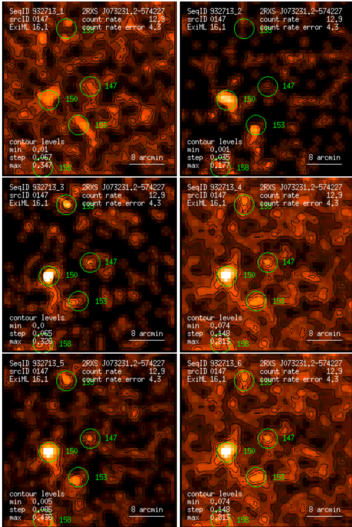
Figure 147: RASS 932713: detection 0147: band rate images, Gaussian filter: (1) PSPC channels 11 – 41, (2) 52 – 90, (3) 91 – 201, (4) 11 – 235, (5) 52 – 201, (6) 11 – 201. Broad band rates in counts/ks. Band rate contour levels in counts/ks/arcmin 2 .
