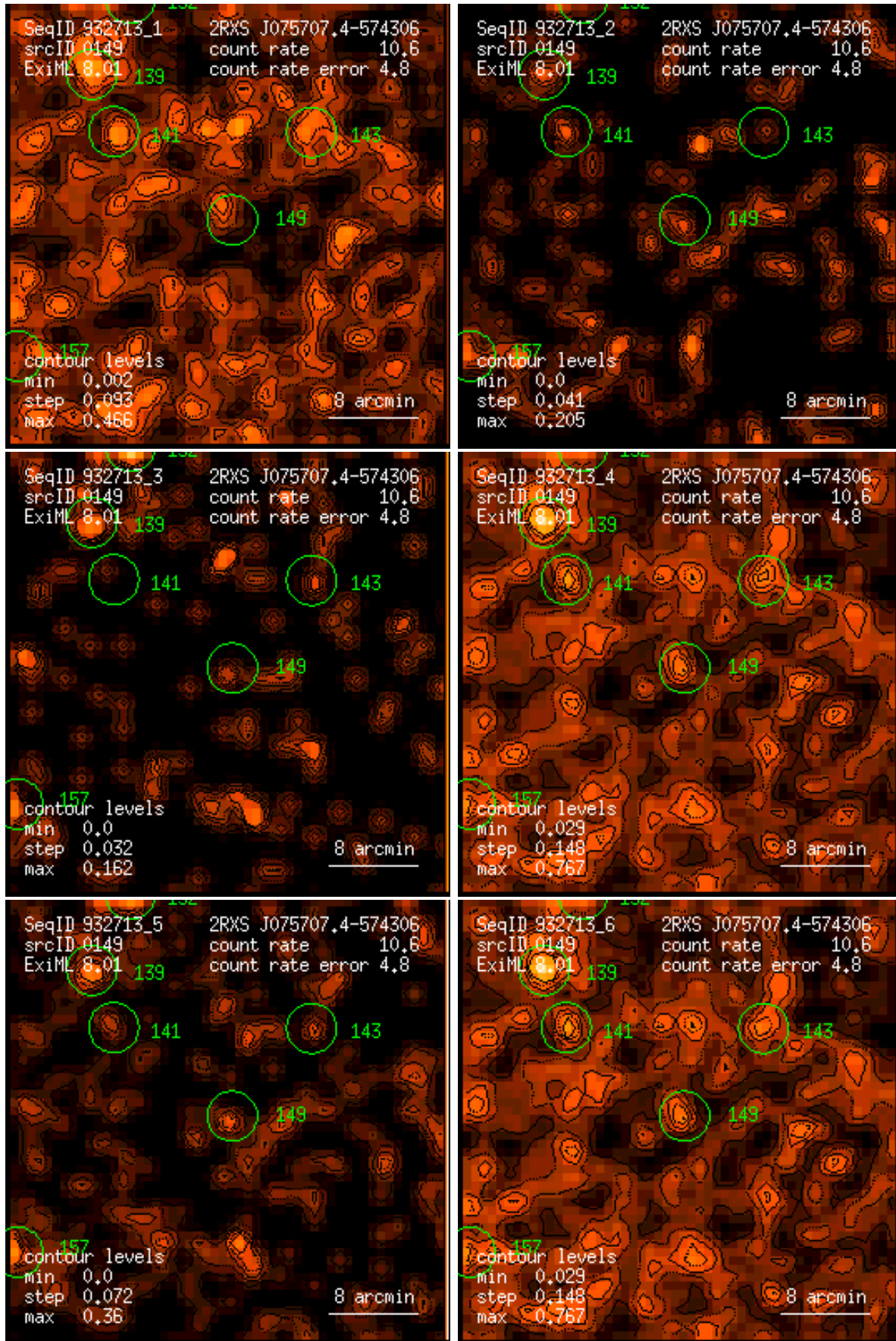
Figure 149: RASS 932713: detection 0149: band rate images, Gaussian filter: (1) PSPC channels 11 – 41, (2) 52 – 90, (3) 91 – 201, (4) 11 – 235, (5) 52 – 201, (6) 11 – 201. Broad band rates in counts/ks. Band rate contour levels in counts/ks/arcmin 2 .
