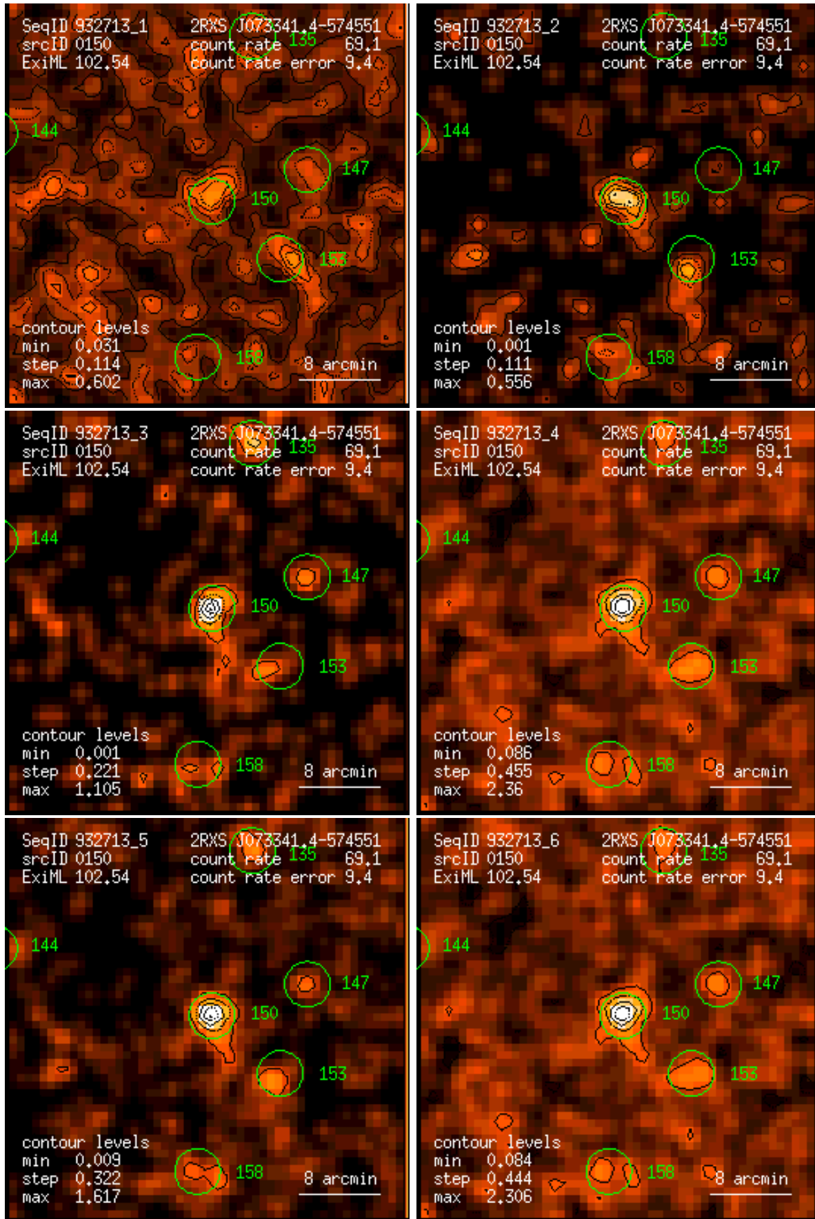
Figure 150: RASS 932713: detection 0150: band rate images, Gaussian filter: (1) PSPC channels 11 – 41, (2) 52 – 90, (3) 91 – 201, (4) 11 – 235, (5) 52 – 201, (6) 11 – 201. Broad band rates in counts/ks. Band rate contour levels in counts/ks/arcmin 2 .
