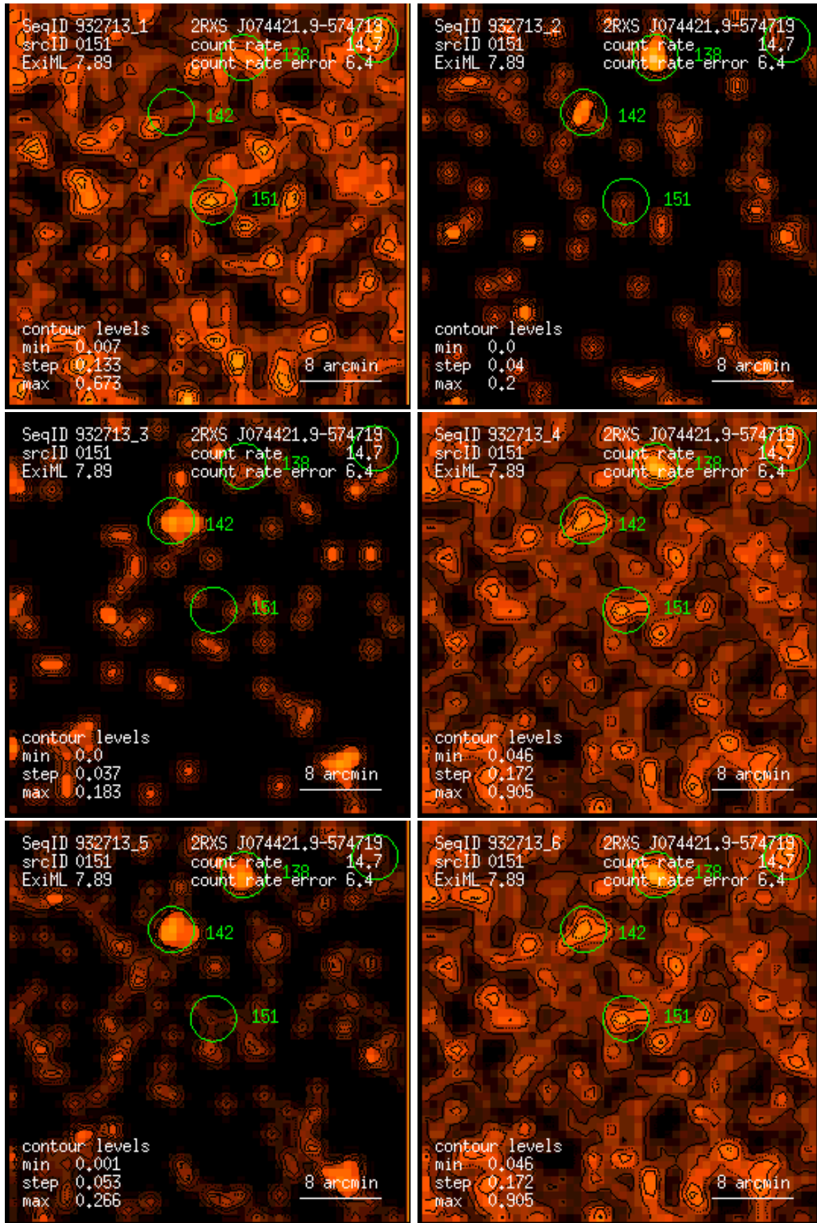
Figure 151: RASS 932713: detection 0151: band rate images, Gaussian filter: (1) PSPC channels 11 – 41, (2) 52 – 90, (3) 91 – 201, (4) 11 – 235, (5) 52 – 201, (6) 11 – 201. Broad band rates in counts/ks. Band rate contour levels in counts/ks/arcmin 2 .
