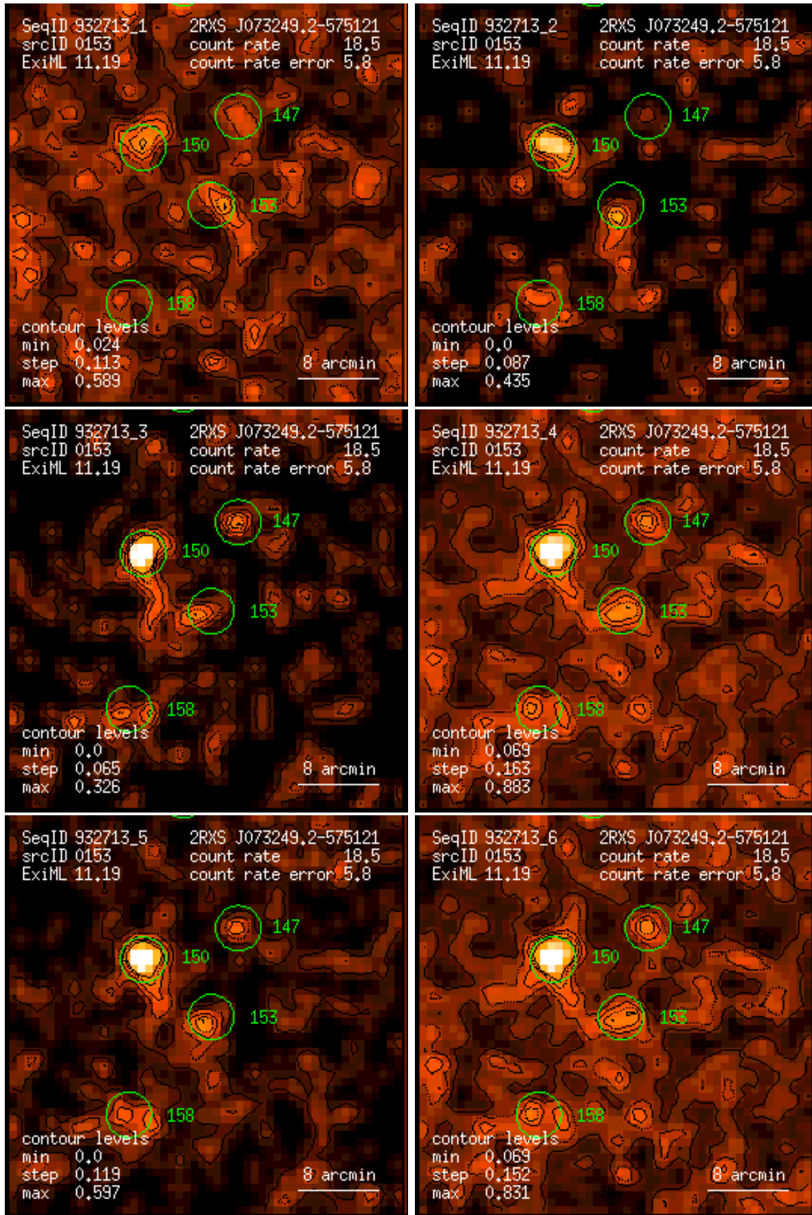
Figure 153: RASS 932713: detection 0153: band rate images, Gaussian filter: (1) PSPC channels 11 – 41, (2) 52 – 90, (3) 91 – 201, (4) 11 – 235, (5) 52 – 201, (6) 11 – 201. Broad band rates in counts/ks. Band rate contour levels in counts/ks/arcmin 2 .
