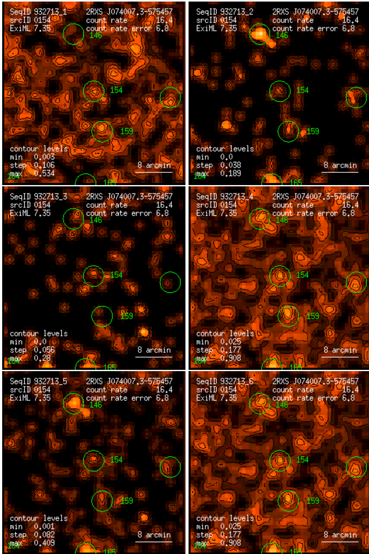
Figure 154: RASS 932713: detection 0154: band rate images, Gaussian filter: (1) PSPC channels 11 – 41, (2) 52 – 90, (3) 91 – 201, (4) 11 – 235, (5) 52 – 201, (6) 11 – 201. Broad band rates in counts/ks. Band rate contour levels in counts/ks/arcmin 2 .
