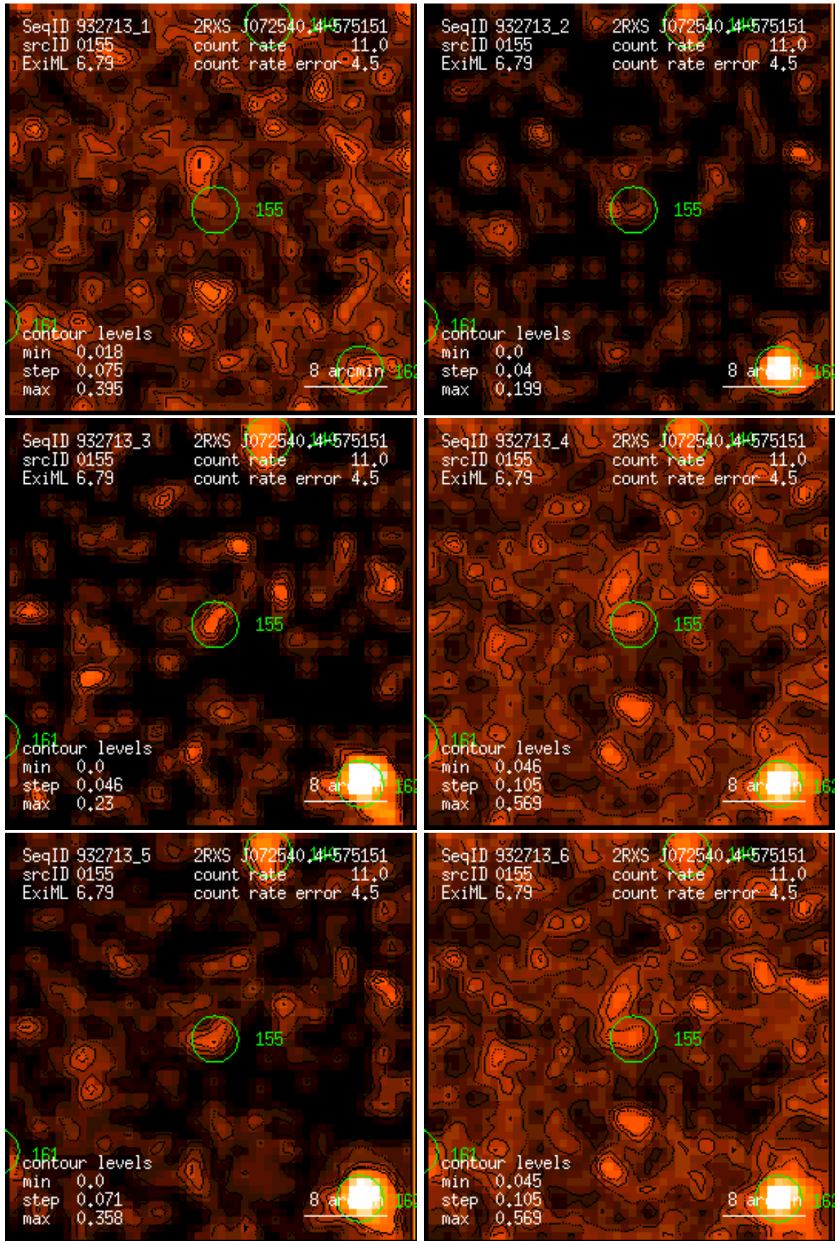
Figure 155: RASS 932713: detection 0155: band rate images, Gaussian filter: (1) PSPC channels 11 – 41, (2) 52 – 90, (3) 91 – 201, (4) 11 – 235, (5) 52 – 201, (6) 11 – 201. Broad band rates in counts/ks. Band rate contour levels in counts/ks/arcmin 2 .
