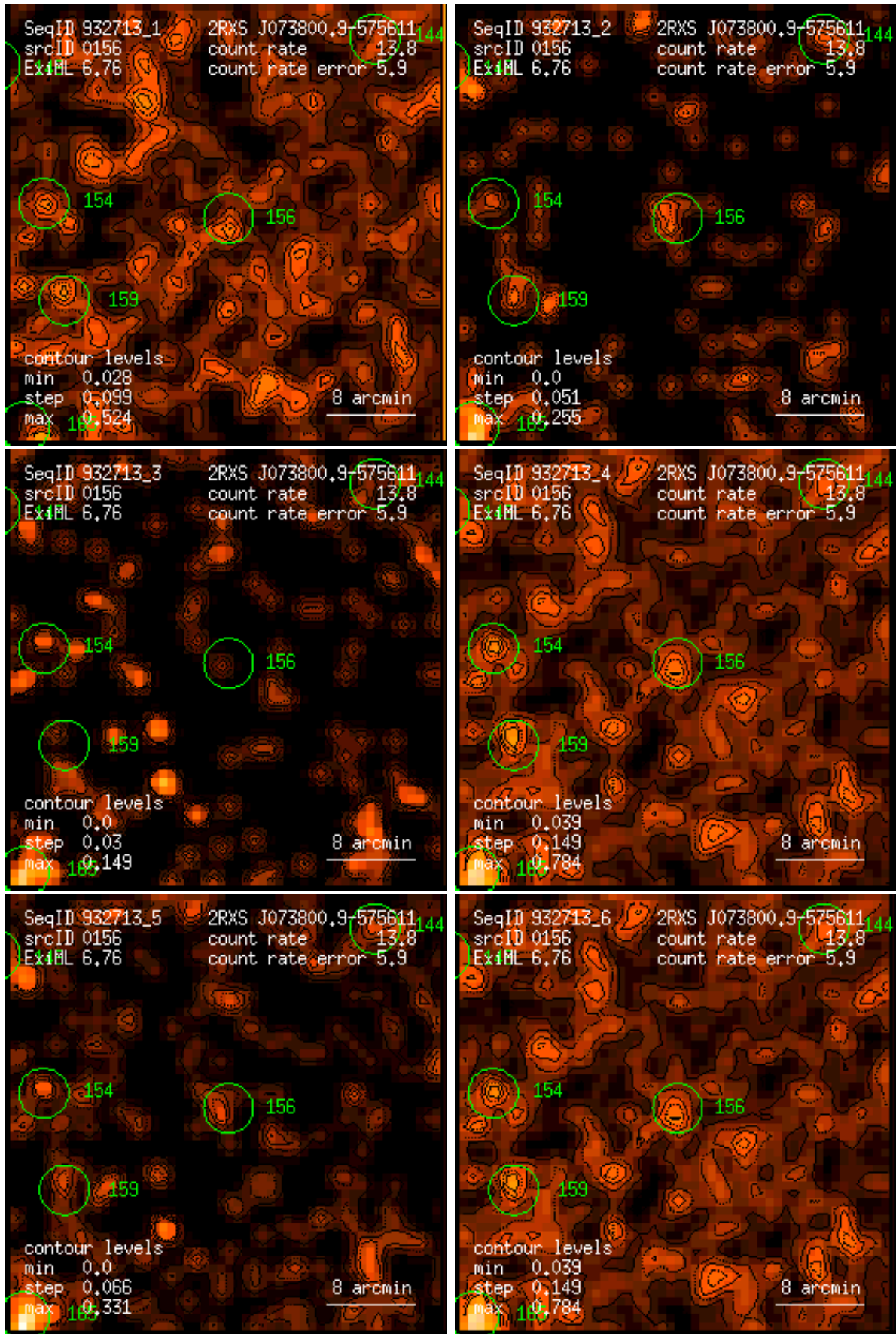
Figure 156: RASS 932713: detection 0156: band rate images, Gaussian filter: (1) PSPC channels 11 – 41, (2) 52 – 90, (3) 91 – 201, (4) 11 – 235, (5) 52 – 201, (6) 11 – 201. Broad band rates in counts/ks. Band rate contour levels in counts/ks/arcmin 2 .
