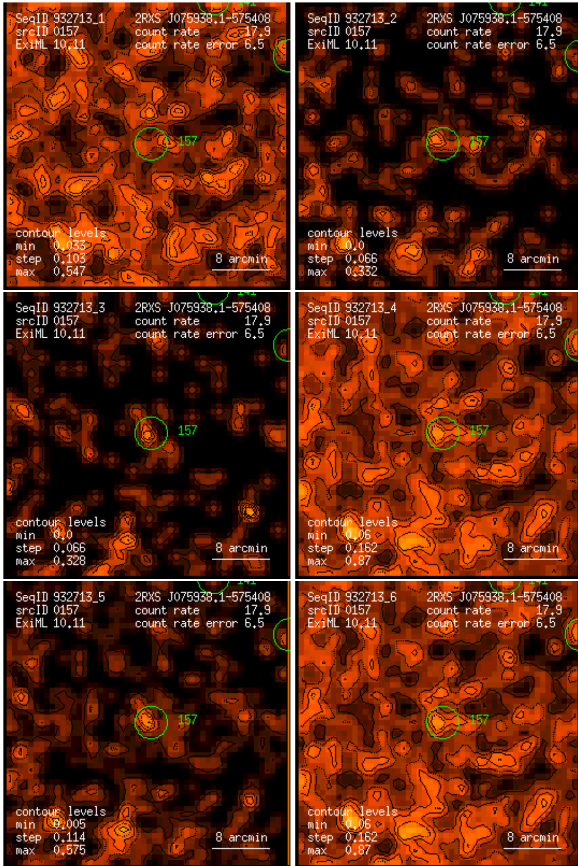
Figure 157: RASS 932713: detection 0157: band rate images, Gaussian filter: (1) PSPC channels 11 – 41, (2) 52 – 90, (3) 91 – 201, (4) 11 – 235, (5) 52 – 201, (6) 11 – 201. Broad band rates in counts/ks. Band rate contour levels in counts/ks/arcmin 2 .
