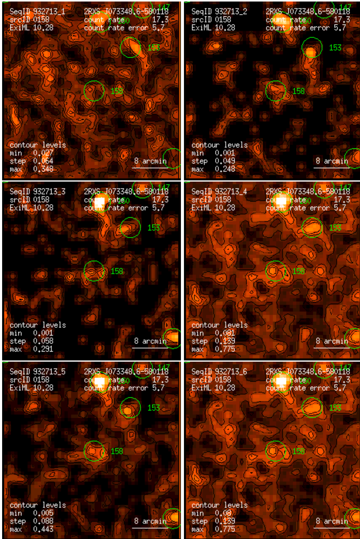
Figure 158: RASS 932713: detection 0158: band rate images, Gaussian filter: (1) PSPC channels 11 – 41, (2) 52 – 90, (3) 91 – 201, (4) 11 – 235, (5) 52 – 201, (6) 11 – 201. Broad band rates in counts/ks. Band rate contour levels in counts/ks/arcmin 2 .
