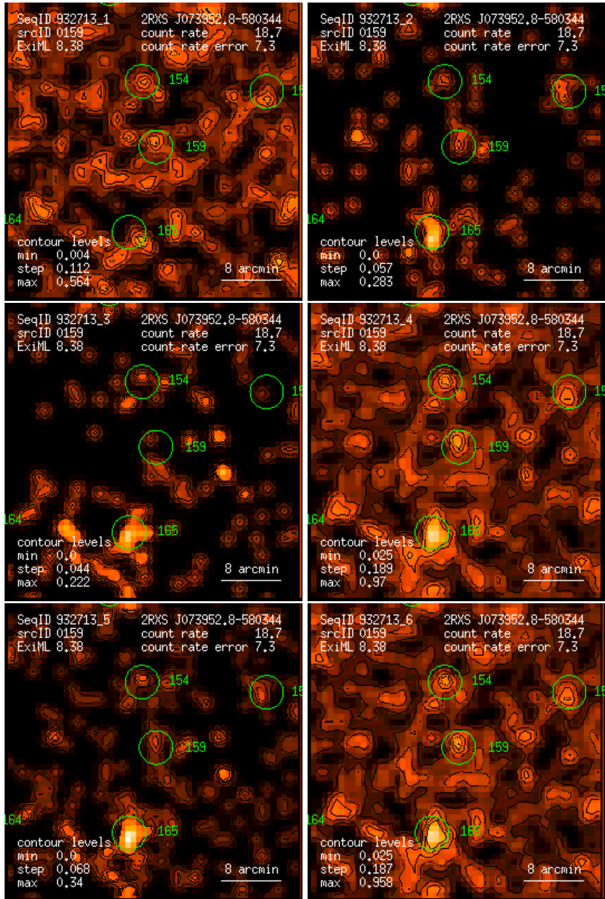
Figure 159: RASS 932713: detection 0159: band rate images, Gaussian filter: (1) PSPC channels 11 – 41, (2) 52 – 90, (3) 91 – 201, (4) 11 – 235, (5) 52 – 201, (6) 11 – 201. Broad band rates in counts/ks. Band rate contour levels in counts/ks/arcmin 2 .
