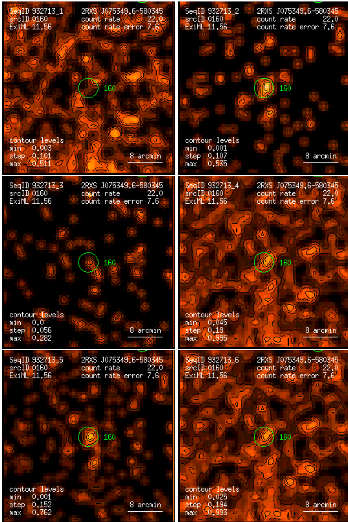
Figure 160: RASS 932713: detection 0160: band rate images, Gaussian filter: (1) PSPC channels 11 – 41, (2) 52 – 90, (3) 91 – 201, (4) 11 – 235, (5) 52 – 201, (6) 11 – 201. Broad band rates in counts/ks. Band rate contour levels in counts/ks/arcmin 2 .
