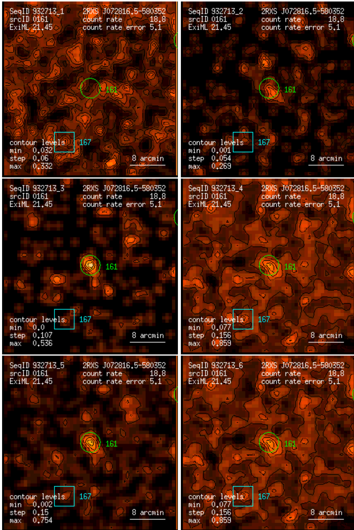
Figure 161: RASS 932713: detection 0161: band rate images, Gaussian filter: (1) PSPC channels 11 – 41, (2) 52 – 90, (3) 91 – 201, (4) 11 – 235, (5) 52 – 201, (6) 11 – 201. Broad band rates in counts/ks. Band rate contour levels in counts/ks/arcmin 2 .
