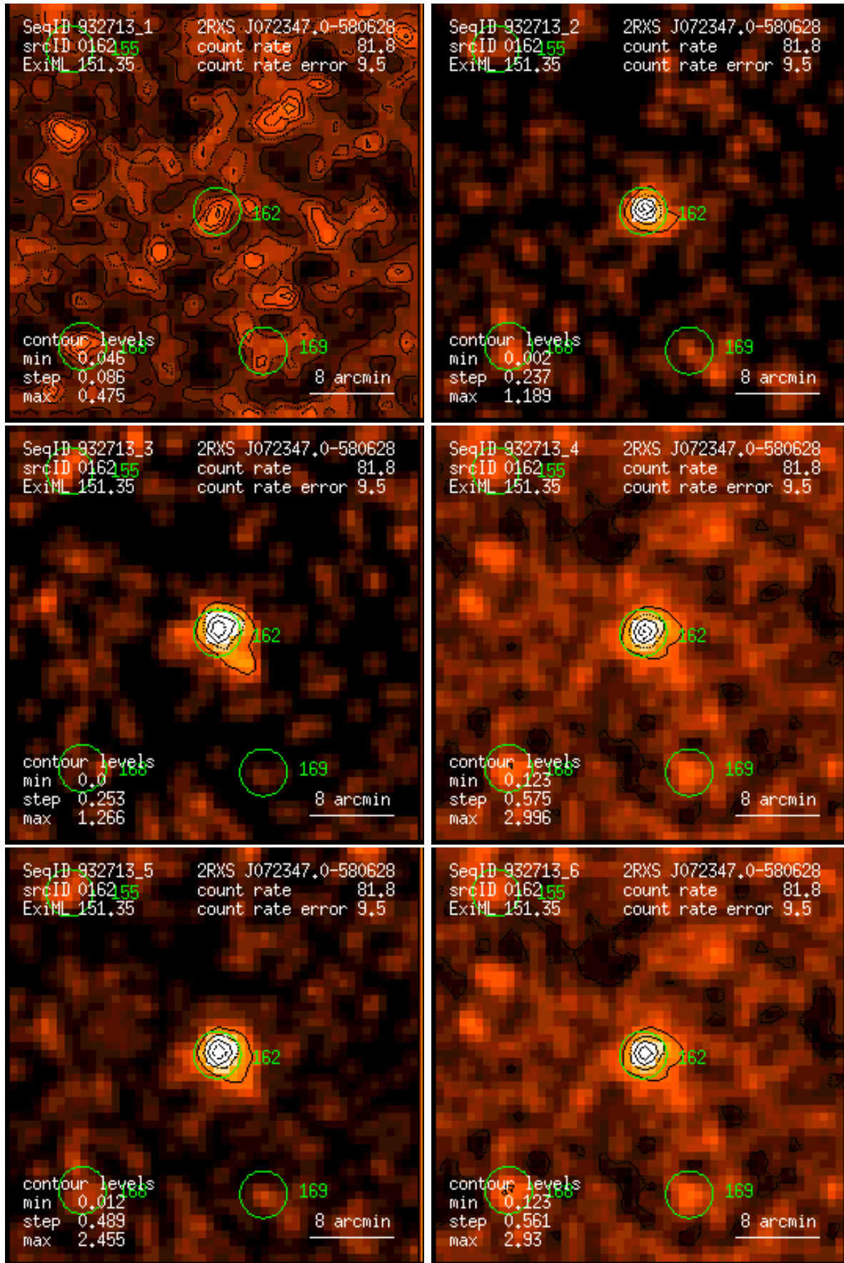
Figure 162: RASS 932713: detection 0162: band rate images, Gaussian filter: (1) PSPC channels 11 – 41, (2) 52 – 90, (3) 91 – 201, (4) 11 – 235, (5) 52 – 201, (6) 11 – 201. Broad band rates in counts/ks. Band rate contour levels in counts/ks/arcmin 2 .
