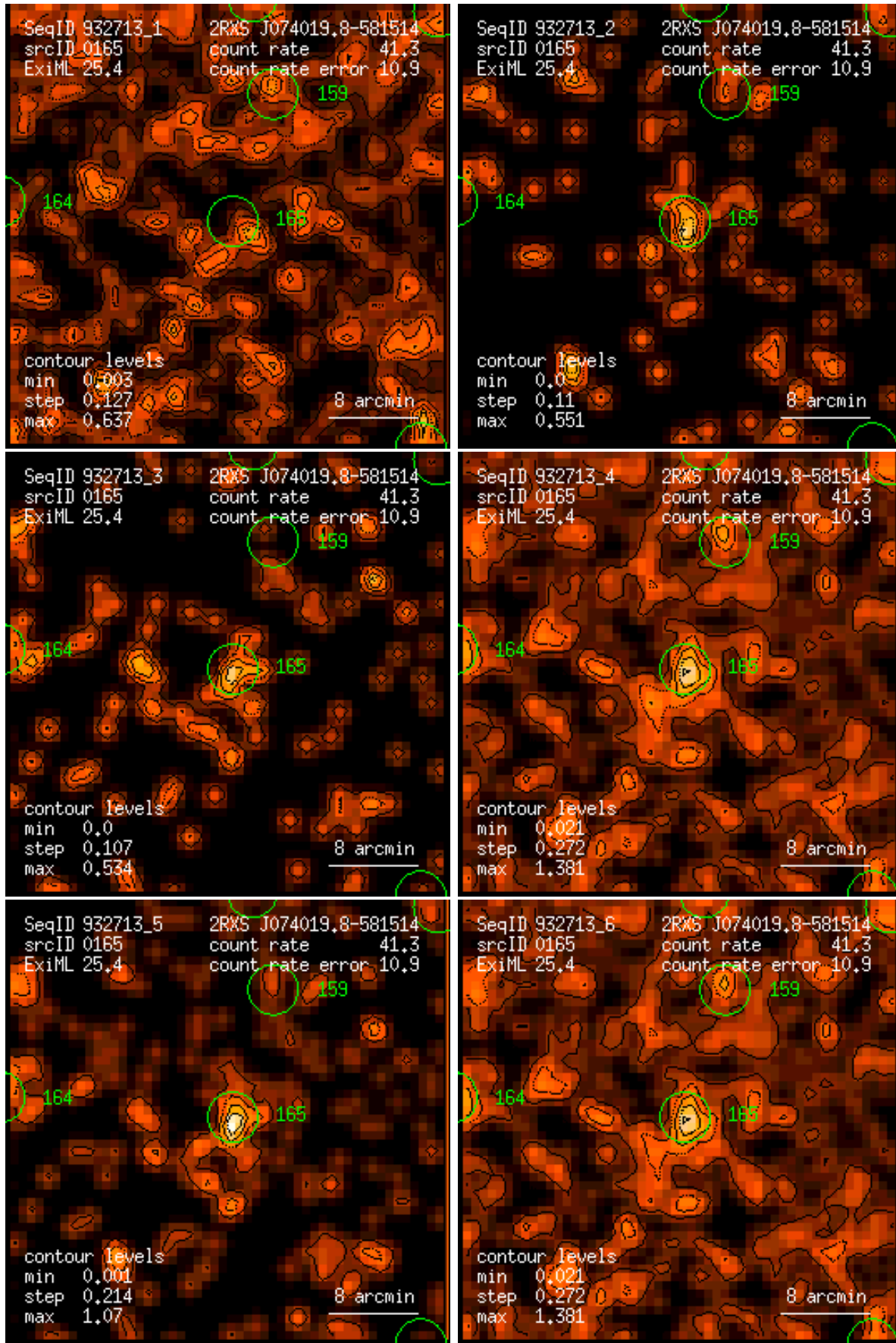
Figure 165: RASS 932713: detection 0165: band rate images, Gaussian filter: (1) PSPC channels 11 – 41, (2) 52 – 90, (3) 91 – 201, (4) 11 – 235, (5) 52 – 201, (6) 11 – 201. Broad band rates in counts/ks. Band rate contour levels in counts/ks/arcmin 2 .
