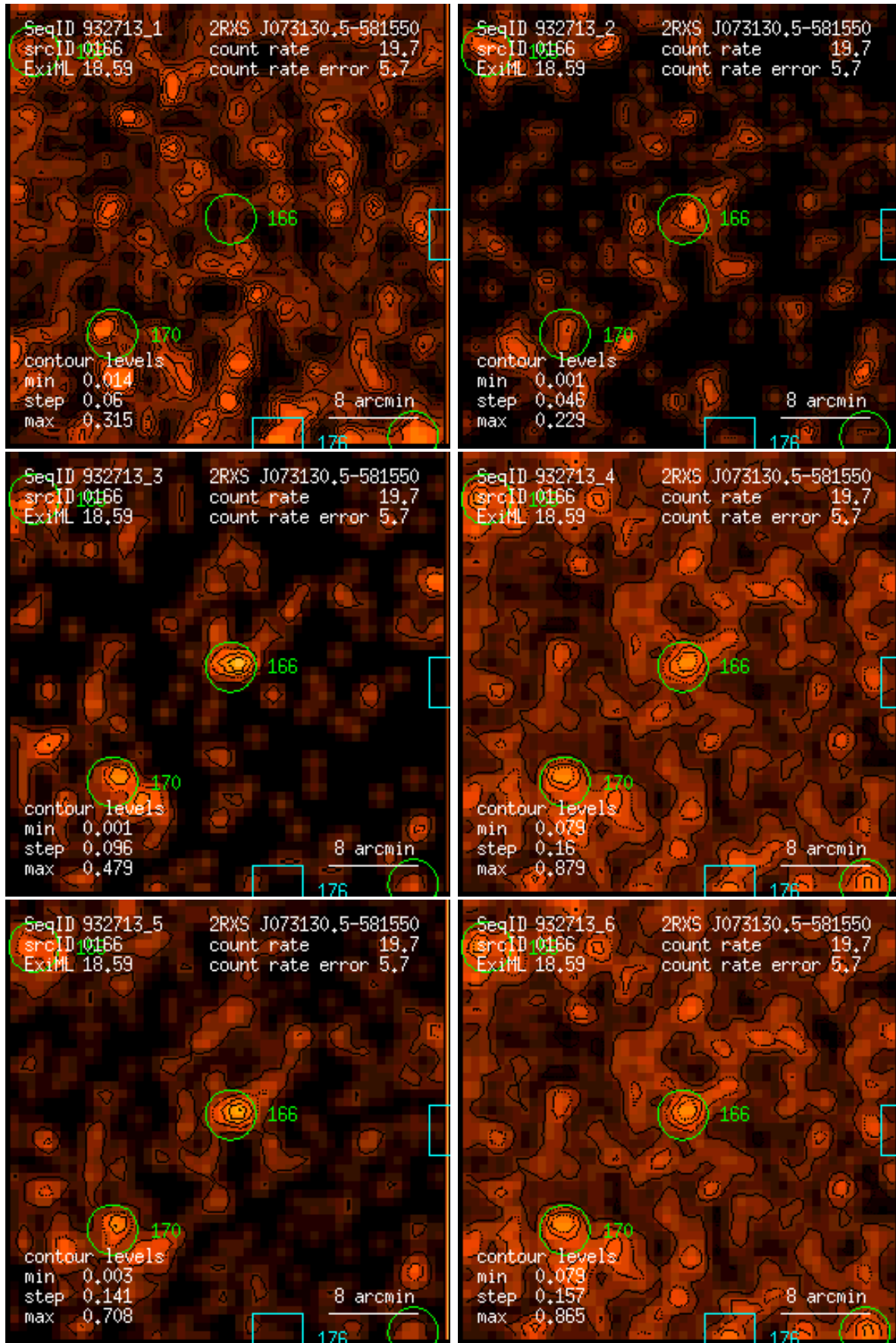
Figure 166: RASS 932713: detection 0166: band rate images, Gaussian filter: (1) PSPC channels 11 – 41, (2) 52 – 90, (3) 91 – 201, (4) 11 – 235, (5) 52 – 201, (6) 11 – 201. Broad band rates in counts/ks. Band rate contour levels in counts/ks/arcmin 2 .
