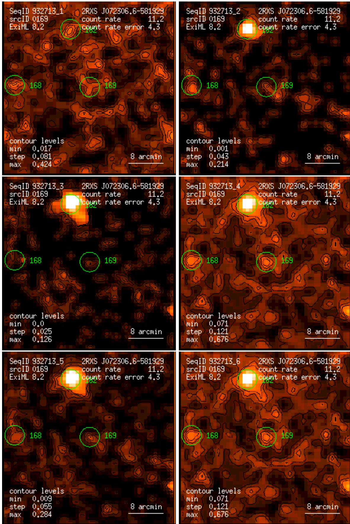
Figure 169: RASS 932713: detection 0169: band rate images, Gaussian filter: (1) PSPC channels 11 – 41, (2) 52 – 90, (3) 91 – 201, (4) 11 – 235, (5) 52 – 201, (6) 11 – 201. Broad band rates in counts/ks. Band rate contour levels in counts/ks/arcmin 2 .
