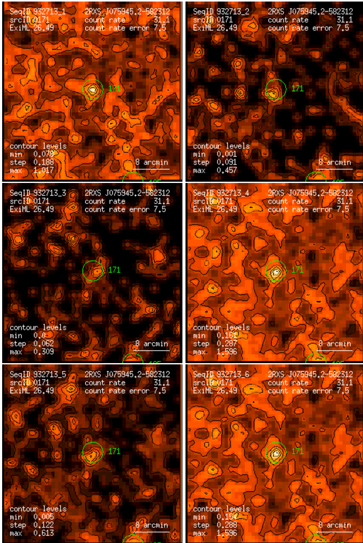
Figure 171: RASS 932713: detection 0171: band rate images, Gaussian filter: (1) PSPC channels 11 – 41, (2) 52 – 90, (3) 91 – 201, (4) 11 – 235, (5) 52 – 201, (6) 11 – 201. Broad band rates in counts/ks. Band rate contour levels in counts/ks/arcmin 2 .
