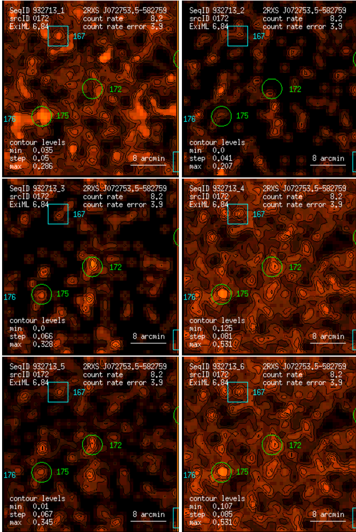
Figure 172: RASS 932713: detection 0172: band rate images, Gaussian filter: (1) PSPC channels 11 – 41, (2) 52 – 90, (3) 91 – 201, (4) 11 – 235, (5) 52 – 201, (6) 11 – 201. Broad band rates in counts/ks. Band rate contour levels in counts/ks/arcmin 2 .
