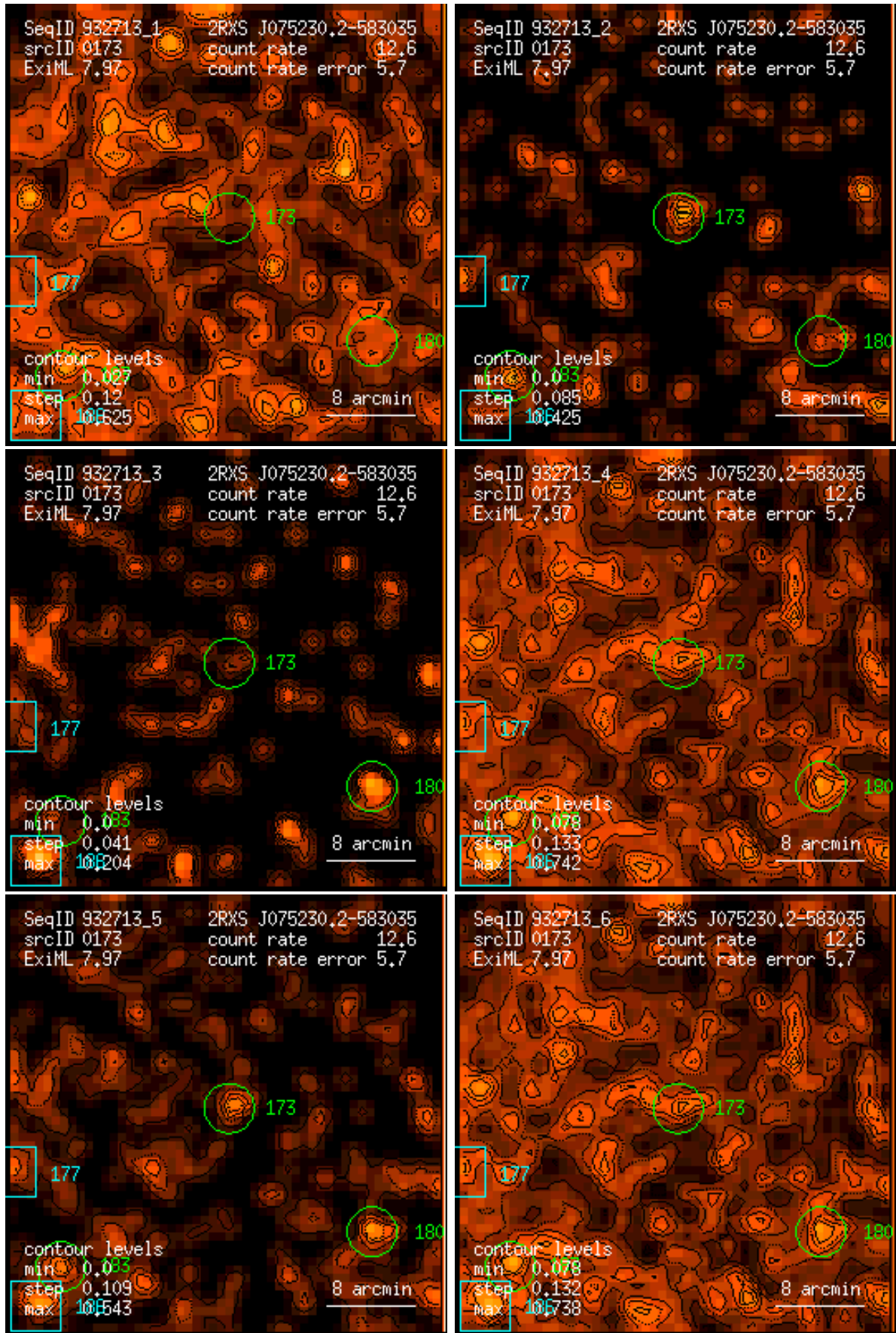
Figure 173: RASS 932713: detection 0173: band rate images, Gaussian filter: (1) PSPC channels 11 – 41, (2) 52 – 90, (3) 91 – 201, (4) 11 – 235, (5) 52 – 201, (6) 11 – 201. Broad band rates in counts/ks. Band rate contour levels in counts/ks/arcmin 2 .
