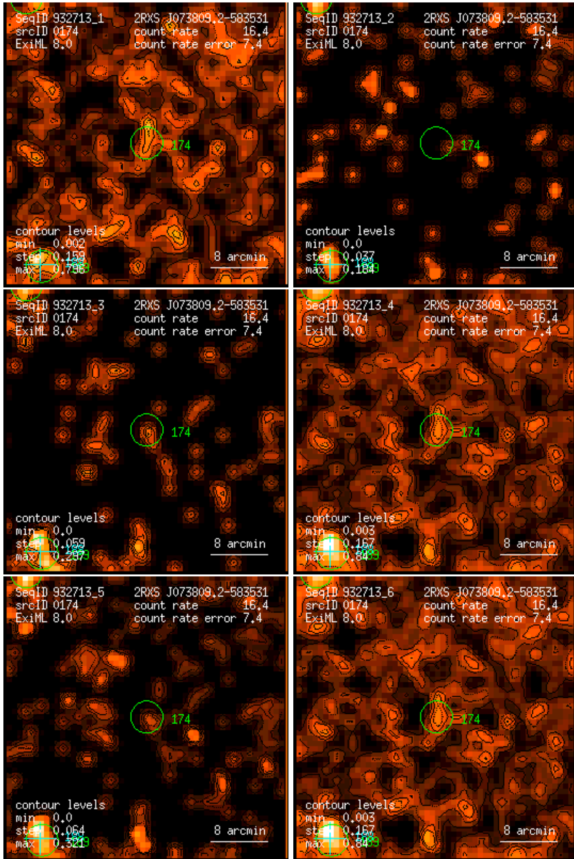
Figure 174: RASS 932713: detection 0174: band rate images, Gaussian filter: (1) PSPC channels 11 – 41, (2) 52 – 90, (3) 91 – 201, (4) 11 – 235, (5) 52 – 201, (6) 11 – 201. Broad band rates in counts/ks. Band rate contour levels in counts/ks/arcmin 2 .
