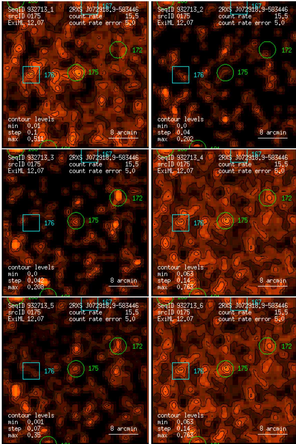
Figure 175: RASS 932713: detection 0175: band rate images, Gaussian filter: (1) PSPC channels 11 – 41, (2) 52 – 90, (3) 91 – 201, (4) 11 – 235, (5) 52 – 201, (6) 11 – 201. Broad band rates in counts/ks. Band rate contour levels in counts/ks/arcmin 2 .
