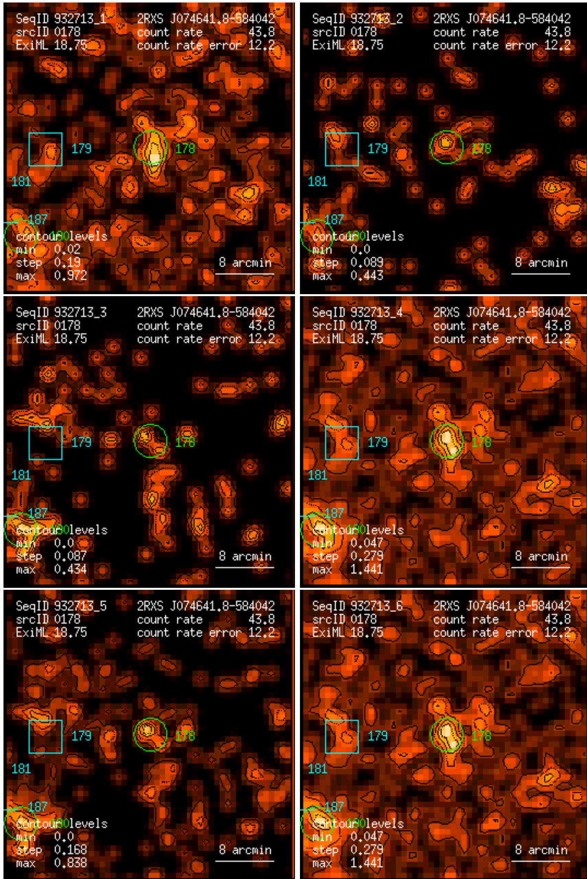
Figure 178: RASS 932713: detection 0178: band rate images, Gaussian filter: (1) PSPC channels 11 – 41, (2) 52 – 90, (3) 91 – 201, (4) 11 – 235, (5) 52 – 201, (6) 11 – 201. Broad band rates in counts/ks. Band rate contour levels in counts/ks/arcmin 2 .
