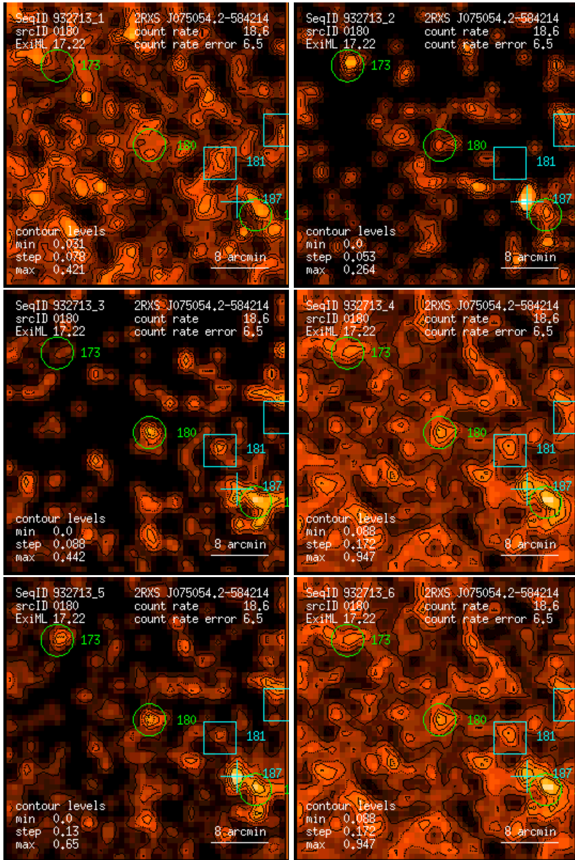
Figure 180: RASS 932713: detection 0180: band rate images, Gaussian filter: (1) PSPC channels 11 – 41, (2) 52 – 90, (3) 91 – 201, (4) 11 – 235, (5) 52 – 201, (6) 11 – 201. Broad band rates in counts/ks. Band rate contour levels in counts/ks/arcmin 2 .
