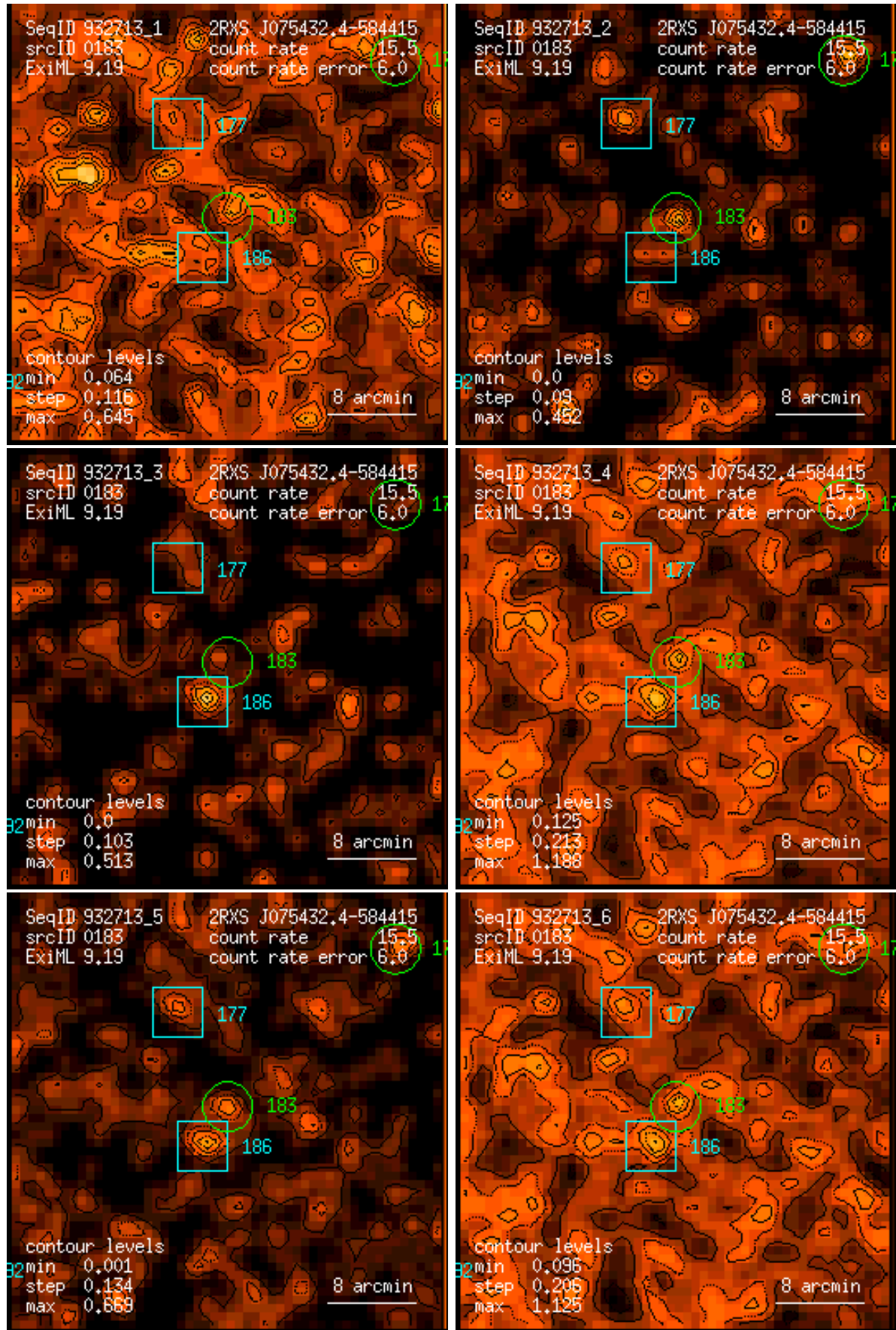
Figure 183: RASS 932713: detection 0183: band rate images, Gaussian filter: (1) PSPC channels 11 – 41, (2) 52 – 90, (3) 91 – 201, (4) 11 – 235, (5) 52 – 201, (6) 11 – 201. Broad band rates in counts/ks. Band rate contour levels in counts/ks/arcmin 2 .
