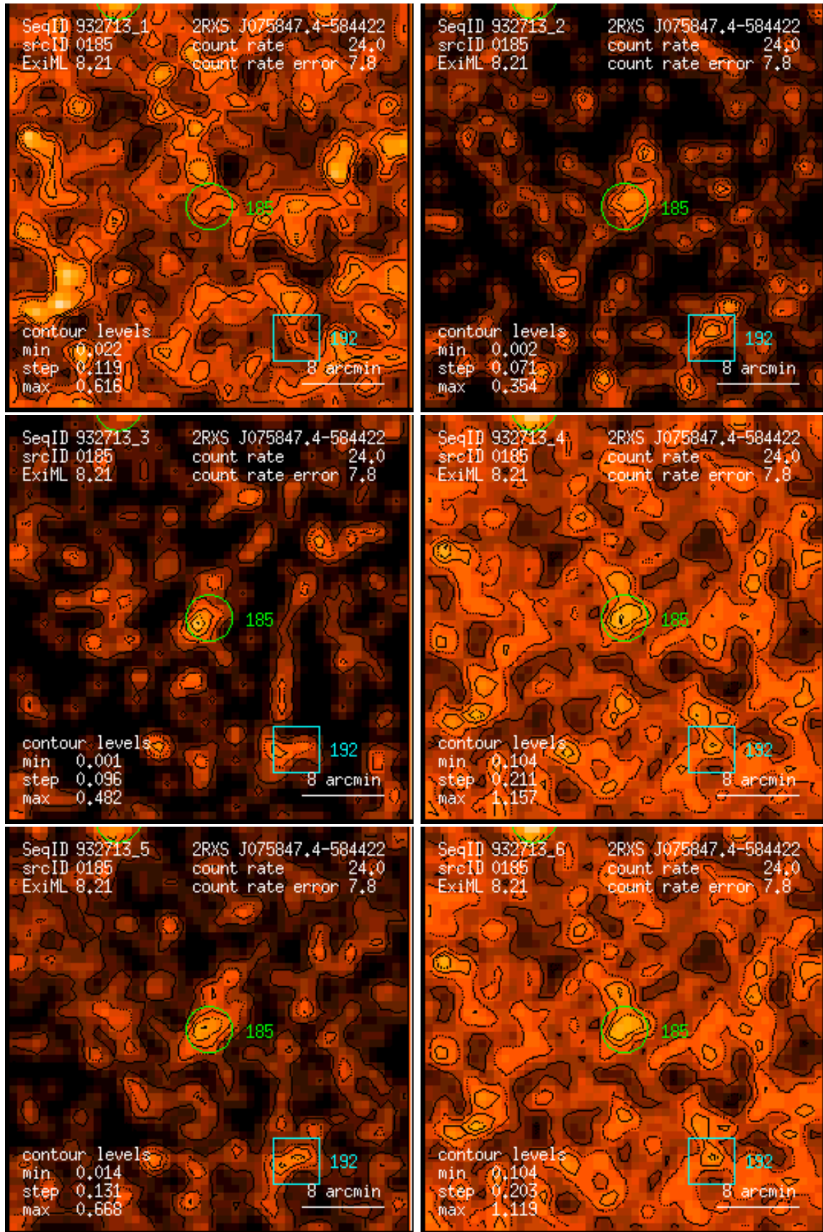
Figure 185: RASS 932713: detection 0185: band rate images, Gaussian filter: (1) PSPC channels 11 – 41, (2) 52 – 90, (3) 91 – 201, (4) 11 – 235, (5) 52 – 201, (6) 11 – 201. Broad band rates in counts/ks. Band rate contour levels in counts/ks/arcmin 2 .
