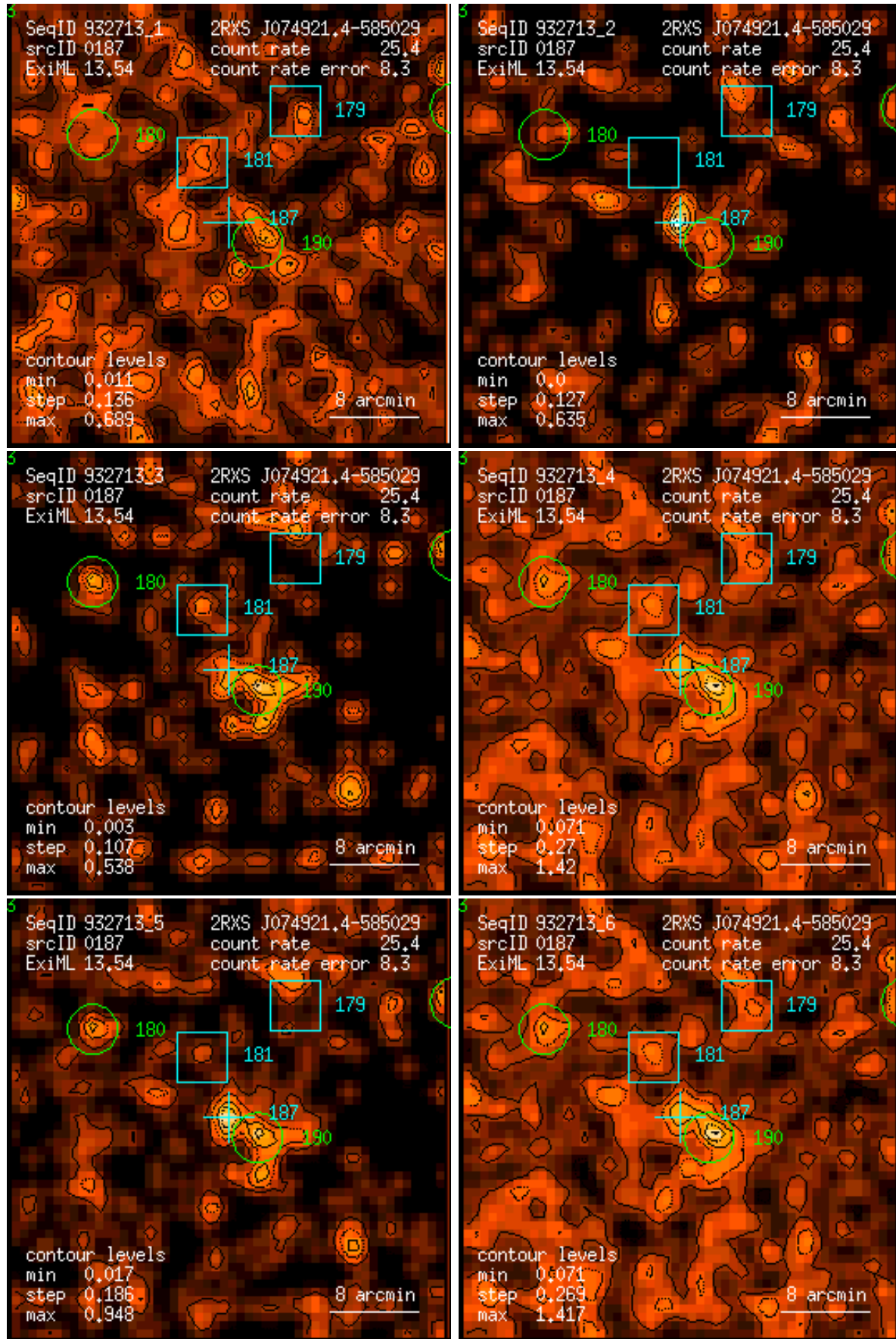
Figure 187: RASS 932713: detection 0187: band rate images, Gaussian filter: (1) PSPC channels 11 – 41, (2) 52 – 90, (3) 91 – 201, (4) 11 – 235, (5) 52 – 201, (6) 11 – 201. Broad band rates in counts/ks. Band rate contour levels in counts/ks/arcmin 2 .
