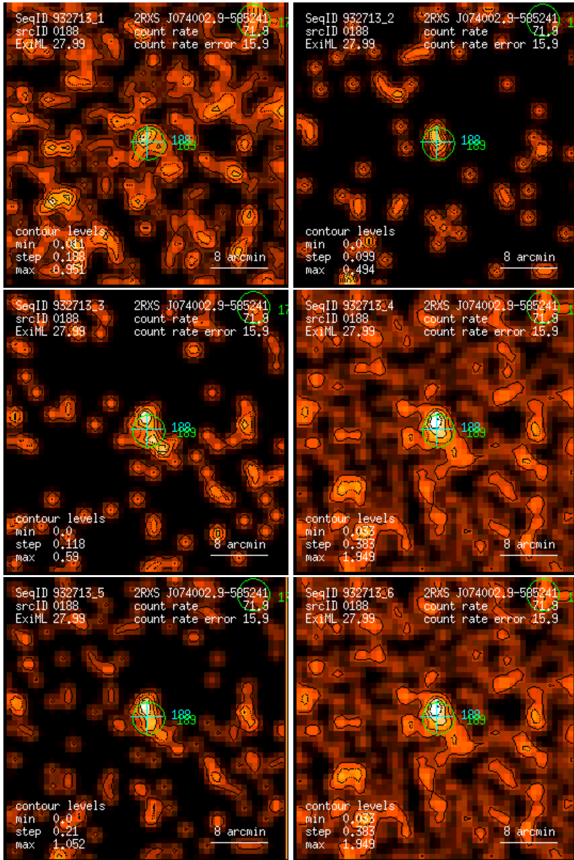
Figure 188: RASS 932713: detection 0188: band rate images, Gaussian filter: (1) PSPC channels 11 – 41, (2) 52 – 90, (3) 91 – 201, (4) 11 – 235, (5) 52 – 201, (6) 11 – 201. Broad band rates in counts/ks. Band rate contour levels in counts/ks/arcmin 2 .
