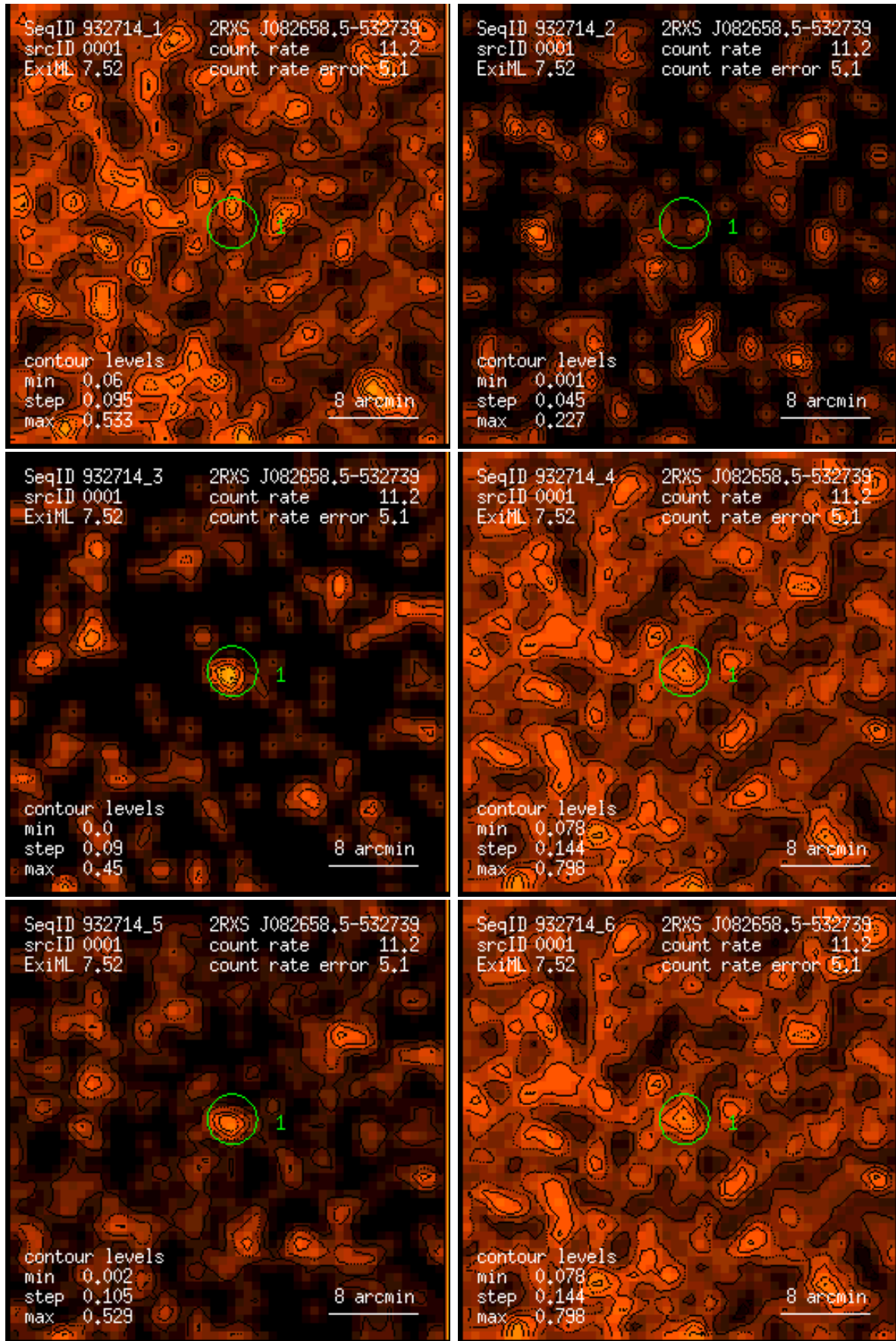
Figure 1: RASS 932714: detection 0001: band rate images, Gaussian filter: (1) PSPC channels 11 – 41, (2) 52 – 90, (3) 91 – 201, (4) 11 – 235, (5) 52 – 201, (6) 11 – 201. Broad band rates in counts/ks. Band rate contour levels in counts/ks/arcmin 2 .
