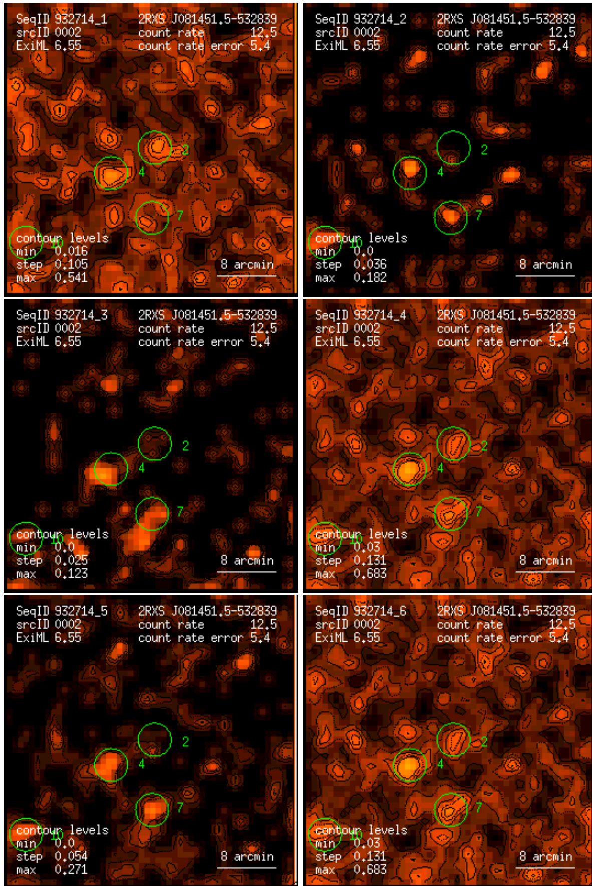
Figure 2: RASS 932714: detection 0002: band rate images, Gaussian filter: (1) PSPC channels 11 – 41, (2) 52 – 90, (3) 91 – 201, (4) 11 – 235, (5) 52 – 201, (6) 11 – 201. Broad band rates in counts/ks. Band rate contour levels in counts/ks/arcmin 2 .
