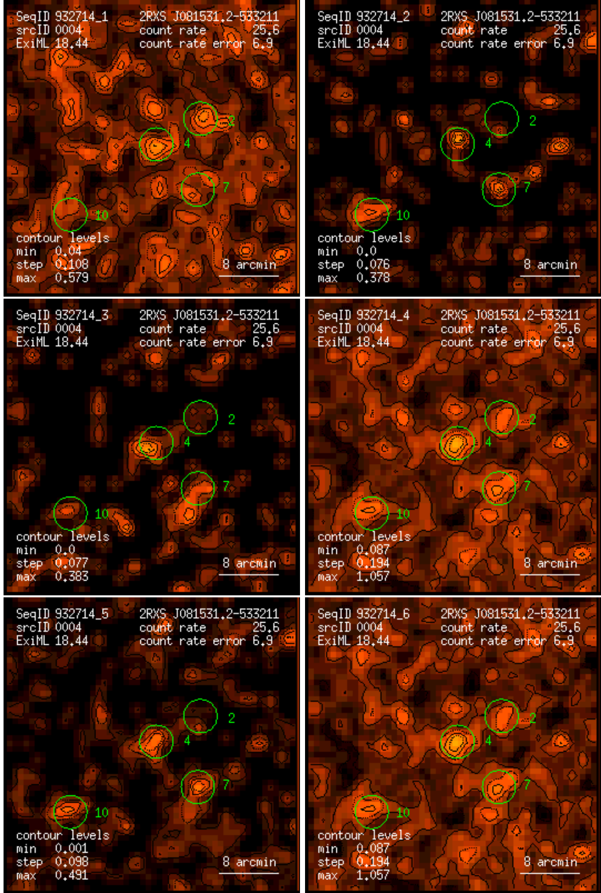
Figure 4: RASS 932714: detection 0004: band rate images, Gaussian filter: (1) PSPC channels 11 – 41, (2) 52 – 90, (3) 91 – 201, (4) 11 – 235, (5) 52 – 201, (6) 11 – 201. Broad band rates in counts/ks. Band rate contour levels in counts/ks/arcmin 2 .
