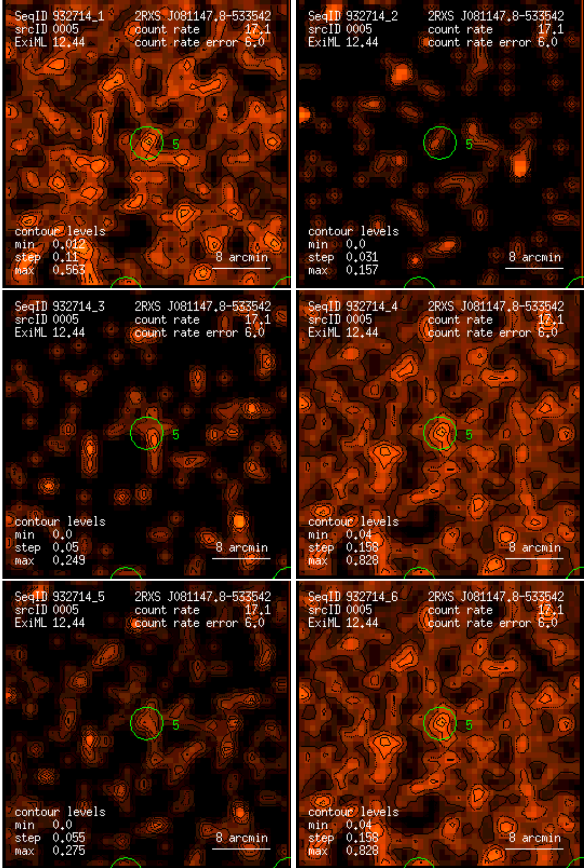
Figure 5: RASS 932714: detection 0005: band rate images, Gaussian filter: (1) PSPC channels 11 – 41, (2) 52 – 90, (3) 91 – 201, (4) 11 – 235, (5) 52 – 201, (6) 11 – 201. Broad band rates in counts/ks. Band rate contour levels in counts/ks/arcmin 2 .
