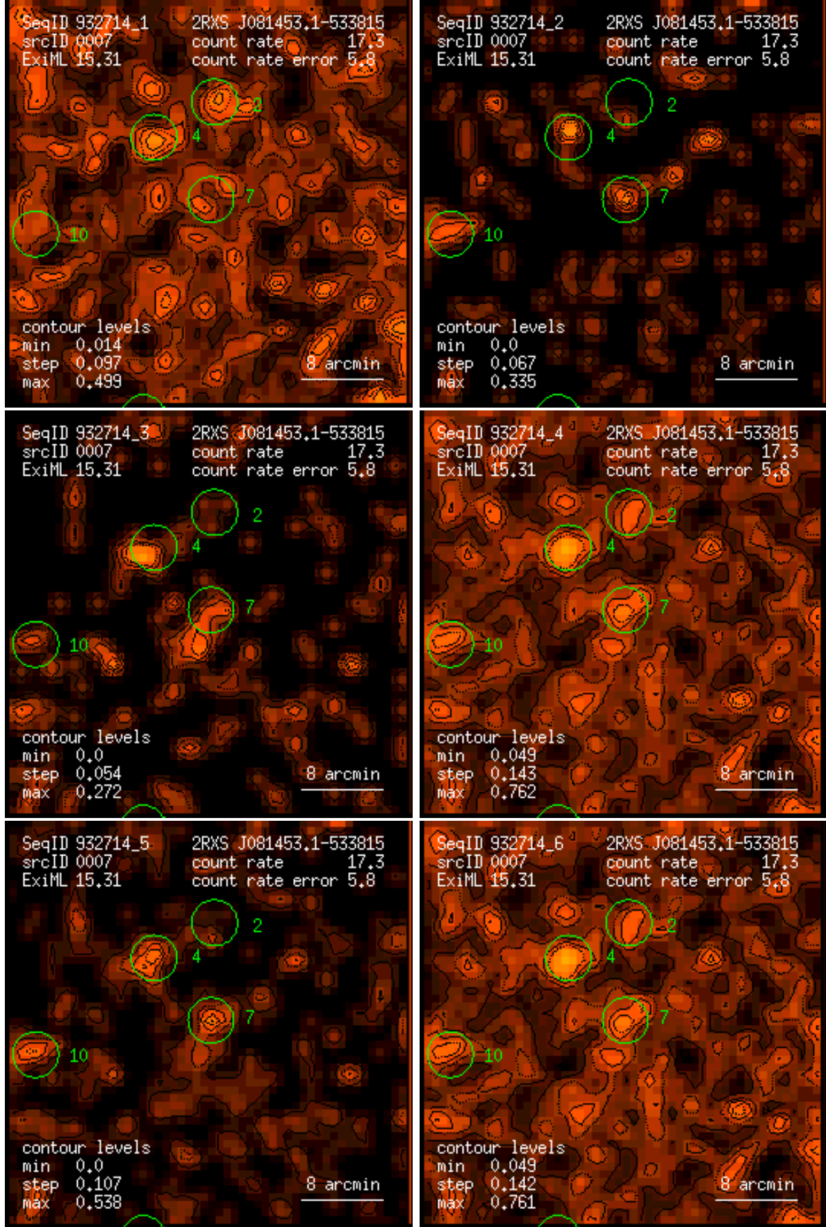
Figure 7: RASS 932714: detection 0007: band rate images, Gaussian filter: (1) PSPC channels 11 – 41, (2) 52 – 90, (3) 91 – 201, (4) 11 – 235, (5) 52 – 201, (6) 11 – 201. Broad band rates in counts/ks. Band rate contour levels in counts/ks/arcmin 2 .
