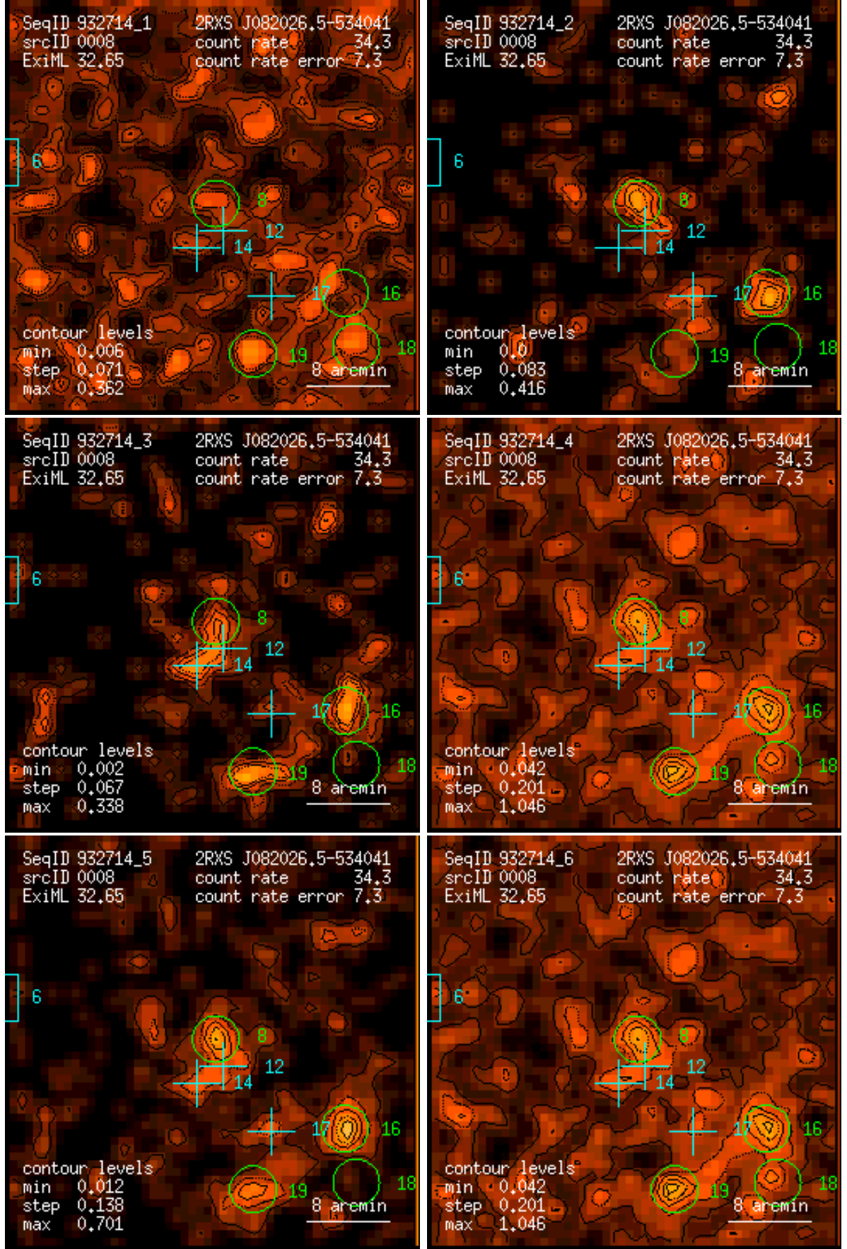
Figure 8: RASS 932714: detection 0008: band rate images, Gaussian filter: (1) PSPC channels 11 – 41, (2) 52 – 90, (3) 91 – 201, (4) 11 – 235, (5) 52 – 201, (6) 11 – 201. Broad band rates in counts/ks. Band rate contour levels in counts/ks/arcmin 2 .
