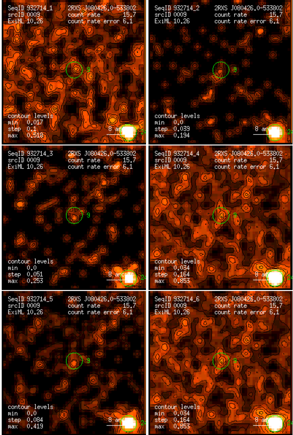
Figure 9: RASS 932714: detection 0009: band rate images, Gaussian filter: (1) PSPC channels 11 – 41, (2) 52 – 90, (3) 91 – 201, (4) 11 – 235, (5) 52 – 201, (6) 11 – 201. Broad band rates in counts/ks. Band rate contour levels in counts/ks/arcmin 2 .
