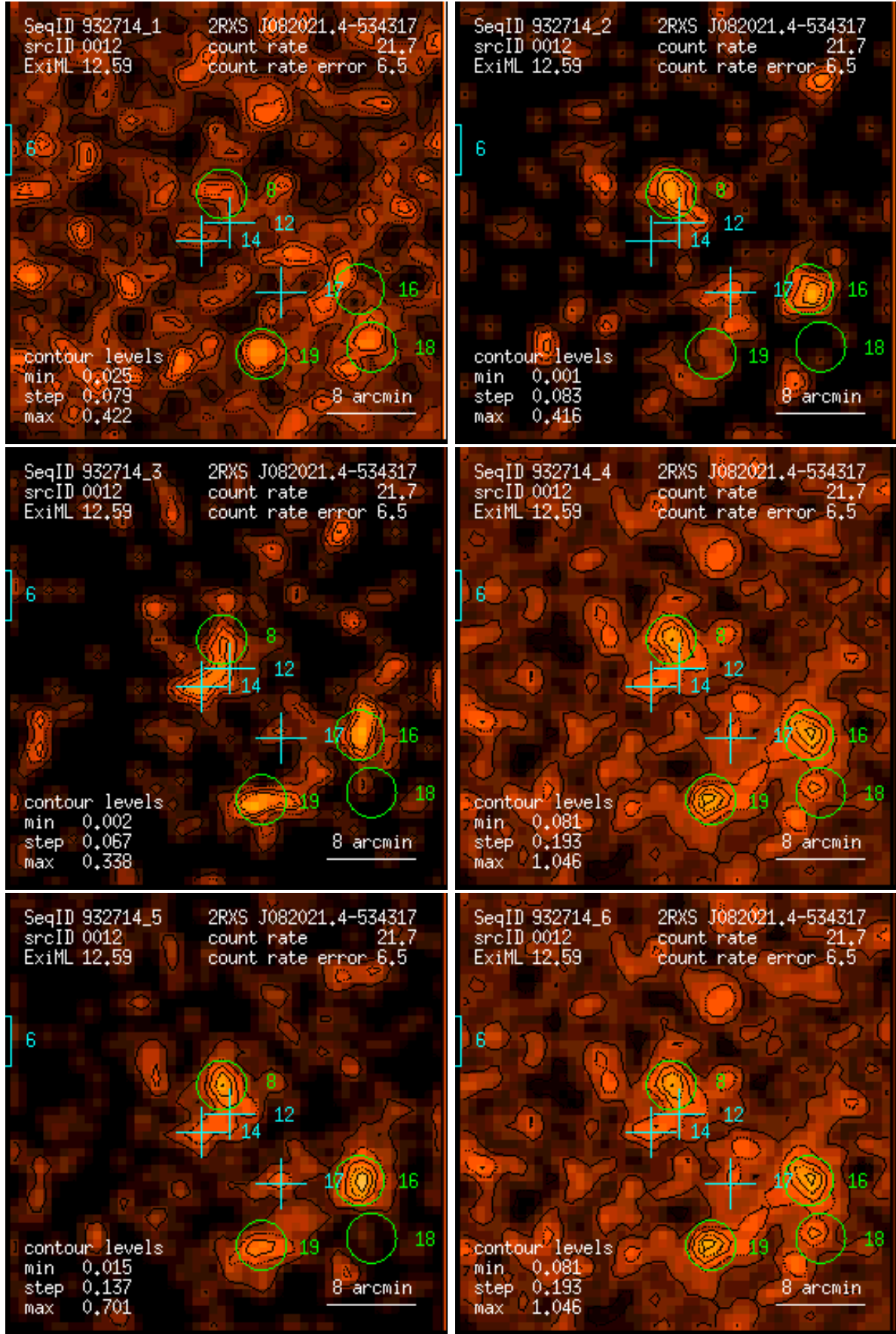
Figure 12: RASS 932714: detection 0012: band rate images, Gaussian filter: (1) PSPC channels 11 – 41, (2) 52 – 90, (3) 91 – 201, (4) 11 – 235, (5) 52 – 201, (6) 11 – 201. Broad band rates in counts/ks. Band rate contour levels in counts/ks/arcmin 2 .
