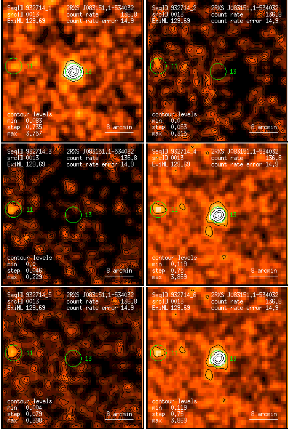
Figure 13: RASS 932714: detection 0013: band rate images, Gaussian filter: (1) PSPC channels 11 – 41, (2) 52 – 90, (3) 91 – 201, (4) 11 – 235, (5) 52 – 201, (6) 11 – 201. Broad band rates in counts/ks. Band rate contour levels in counts/ks/arcmin 2 .
