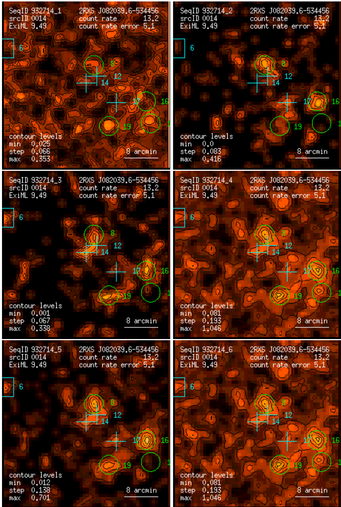
Figure 14: RASS 932714: detection 0014: band rate images, Gaussian filter: (1) PSPC channels 11 – 41, (2) 52 – 90, (3) 91 – 201, (4) 11 – 235, (5) 52 – 201, (6) 11 – 201. Broad band rates in counts/ks. Band rate contour levels in counts/ks/arcmin 2 .
