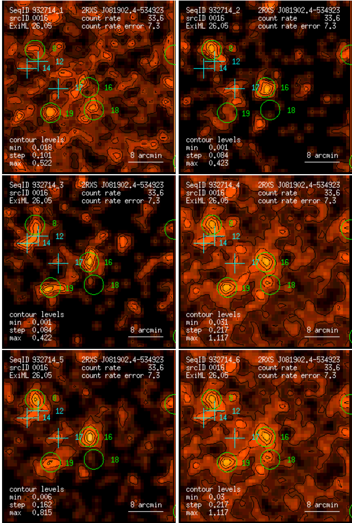
Figure 16: RASS 932714: detection 0016: band rate images, Gaussian filter: (1) PSPC channels 11 – 41, (2) 52 – 90, (3) 91 – 201, (4) 11 – 235, (5) 52 – 201, (6) 11 – 201. Broad band rates in counts/ks. Band rate contour levels in counts/ks/arcmin 2 .
