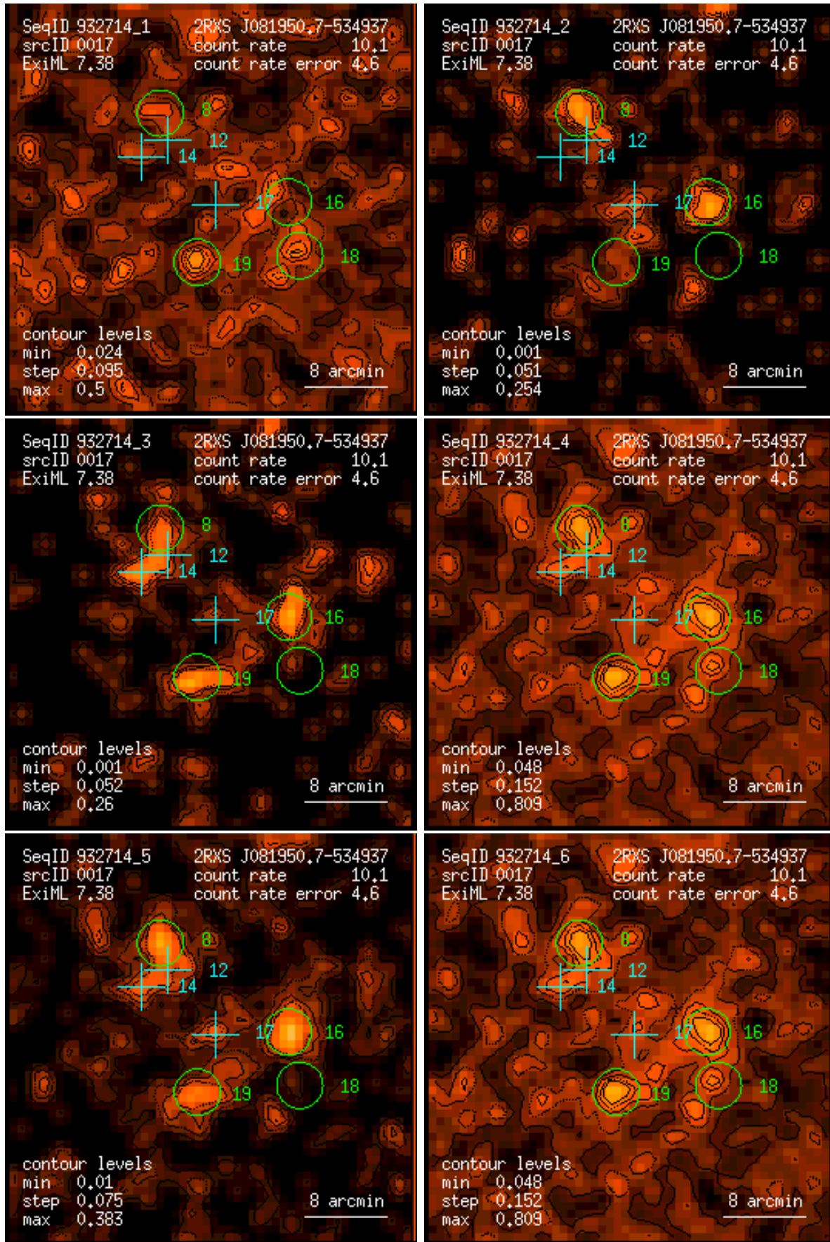
Figure 17: RASS 932714: detection 0017: band rate images, Gaussian filter: (1) PSPC channels 11 – 41, (2) 52 – 90, (3) 91 – 201, (4) 11 – 235, (5) 52 – 201, (6) 11 – 201. Broad band rates in counts/ks. Band rate contour levels in counts/ks/arcmin 2 .
