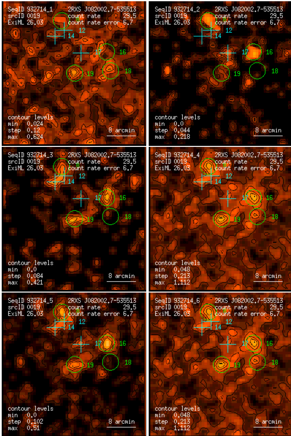
Figure 19: RASS 932714: detection 0019: band rate images, Gaussian filter: (1) PSPC channels 11 – 41, (2) 52 – 90, (3) 91 – 201, (4) 11 – 235, (5) 52 – 201, (6) 11 – 201. Broad band rates in counts/ks. Band rate contour levels in counts/ks/arcmin 2 .
