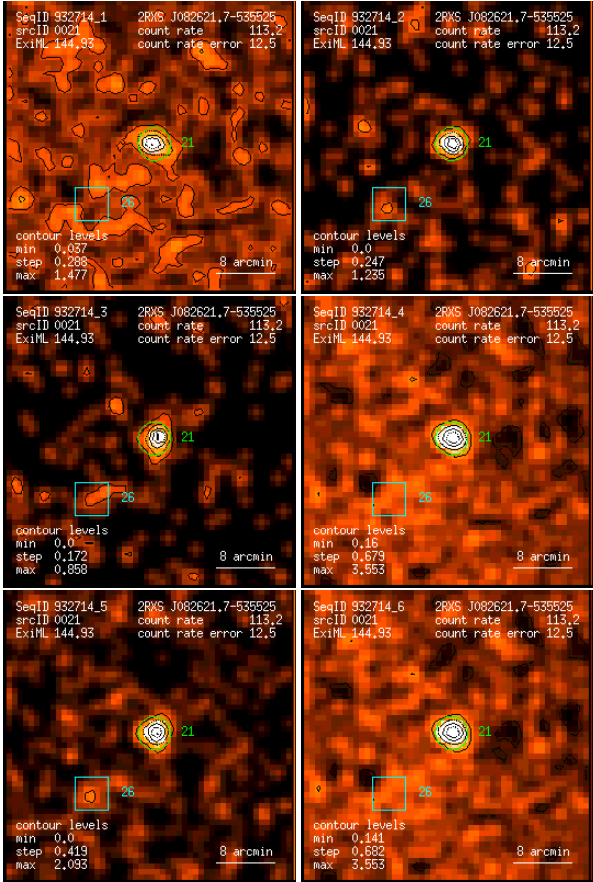
Figure 21: RASS 932714: detection 0021: band rate images, Gaussian filter: (1) PSPC channels 11 – 41, (2) 52 – 90, (3) 91 – 201, (4) 11 – 235, (5) 52 – 201, (6) 11 – 201. Broad band rates in counts/ks. Band rate contour levels in counts/ks/arcmin 2 .
