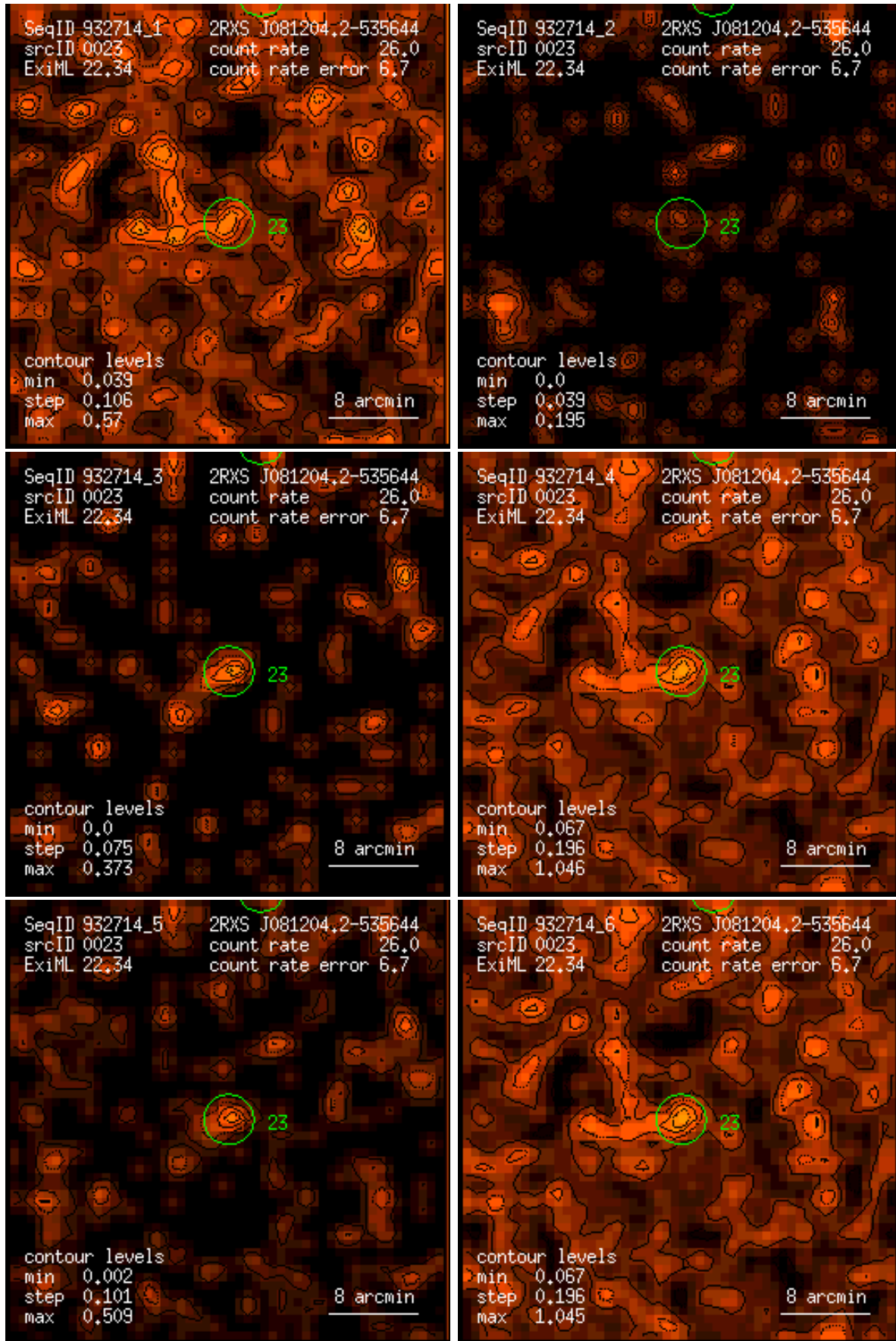
Figure 23: RASS 932714: detection 0023: band rate images, Gaussian filter: (1) PSPC channels 11 – 41, (2) 52 – 90, (3) 91 – 201, (4) 11 – 235, (5) 52 – 201, (6) 11 – 201. Broad band rates in counts/ks. Band rate contour levels in counts/ks/arcmin 2 .
